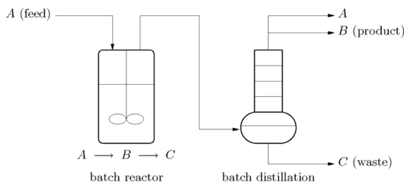
Figure 1. Task network of a two-stage batch process.
