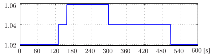
Figure 6: Tap changer position n_T .
