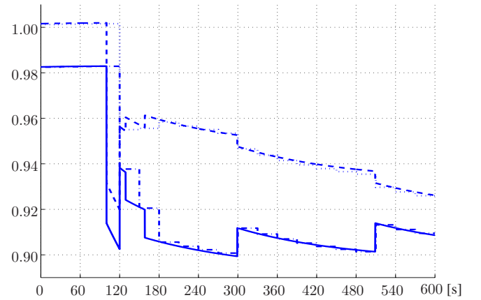
Figure 4: Bus voltages: V_{3m} of the nonlinear model: solid; V_{3m} of the MLD model: dash-dotted; V_{4m} of the nonlinear model: dashed; V_{4m} of the MLD model: dotted.
