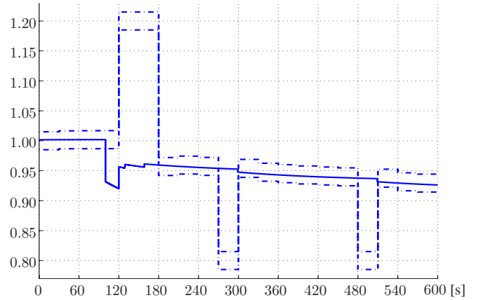
Figure 5: Voltages at bus 4: The tolerance band around V_{4m,ref} is bounded by dash-dotted lines, V_{4m} is a straight line.
