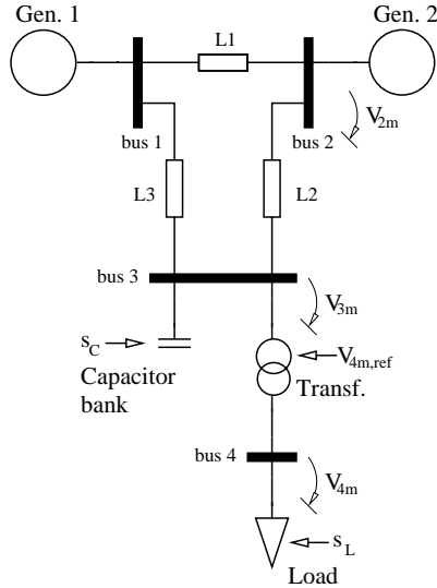
Figure 1: Example power system.
