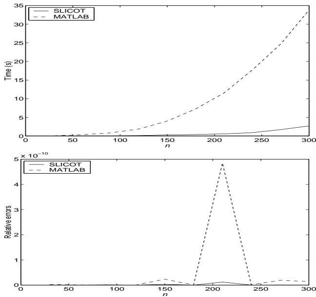
Figure 3: SLICOT slstei versus MATLAB dlyap for random Stein equations with A in real Schur form, n = 30 : 30 : 300 . Timing (top) and relative errors (bottom) comparisons.
