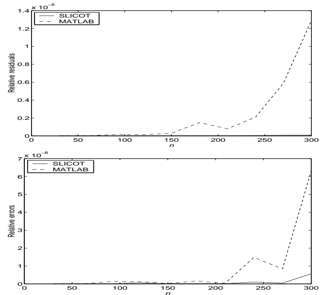
Figure 2: SLICOT slstei versus MATLAB dlyap for random Stein equations with n = 30 : 30 : 300 . Relative residuals (top) and relative errors (bottom) comparisons.
