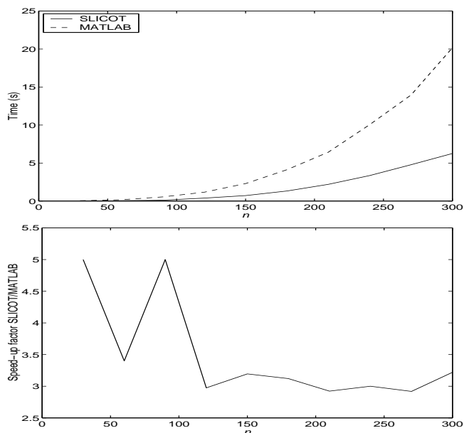
Figure 6: SLICOT slylv versus MATLAB lyap for random Sylvester equations, n = 30 : 30 : 300 , m = n/2 . Timing comparison (top) and speed-up factor (bottom).
