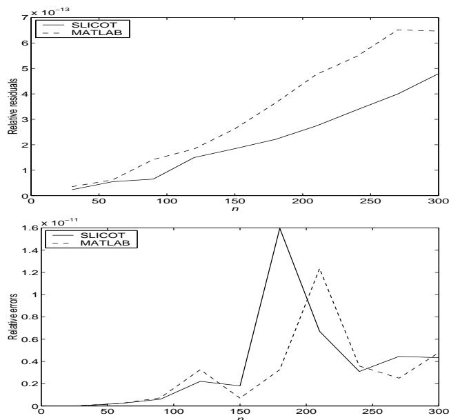
Figure 7: SLICOT slylv versus MATLAB lyap for random Sylvester equations with n = 30 : 30 : 300 , m = n/2 . Relative residuals (top) and relative errors (bottom) comparisons.
