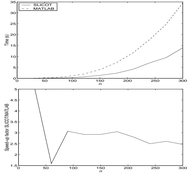
Figure 1: SLICOT slstei versus MATLAB dlyap for random Stein equations with n = 30 : 30 : 300 . Timing comparison (top) and speed-up factor (bottom).
