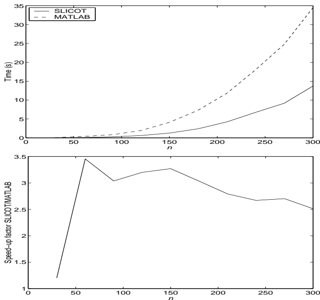
Figure 4: SLICOT slyap versus MATLAB lyap for random Lyapunov equations with n = 30 : 30 : 300 . Timing comparison (top) and speed-up factor (bottom).
