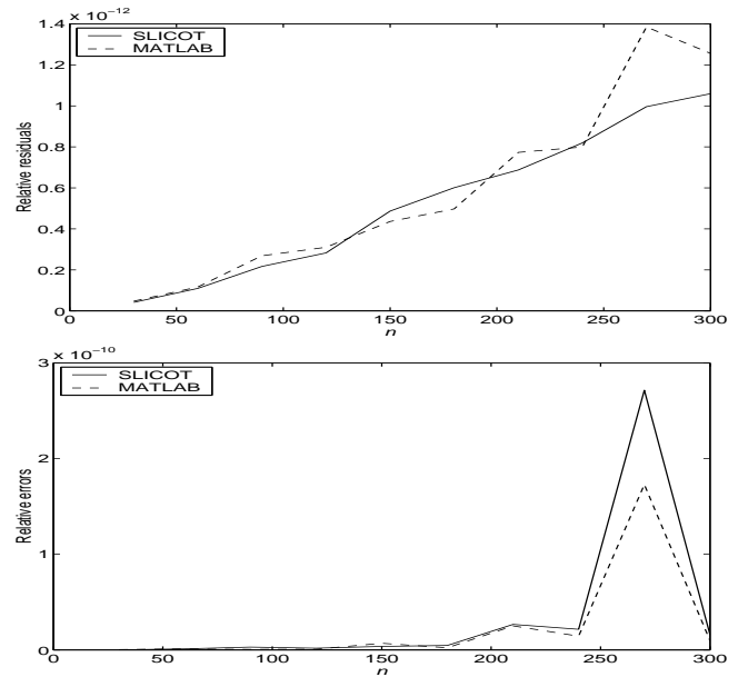
Figure 5: SLICOT slyap versus MATLAB lyap for random Lyapunov equations with n = 30 : 30 : 300 . Relative residuals (top) and relative errors (bottom) comparisons.
