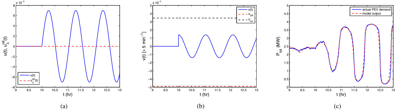
Fig. 4. Case 1, corresponding to Section III-A. The deadband moves slowly and all chargers remain within the limits.
