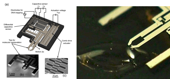
Fig. 1. Silicon nanotweezers
