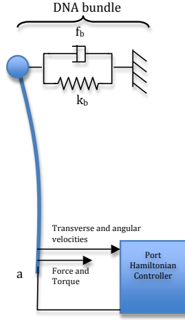
Fig. 2. DNA manipulation through port Hamiltonian control
