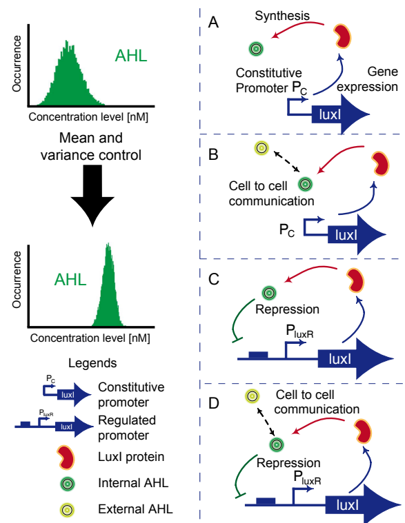
Fig. 1. Different architectures for controlling the AHL distribution across a population. The core principle is to use the P_{luxR} promoter as an interface to control the production of LuxI (thus modulating AHL and the cell-to-cell communication). (A) Open loop production of LuxI without communication. (B) Open loop production of LuxI with communication. (C) Feedback-regulated production of LuxI without communication. (D) Feedback-regulated production of LuxI with communication.
