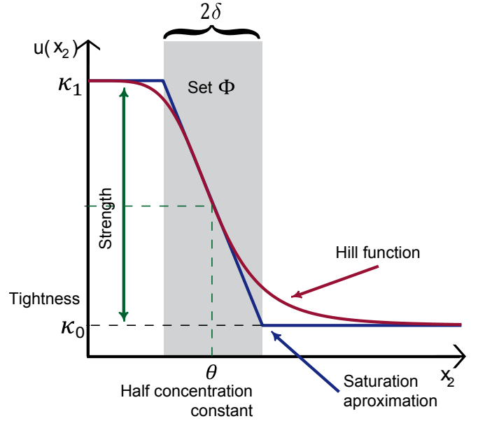
Fig. 3. Characteristic of the promoter. Hill function and its piecewise affine approximation for n = 5 , \theta = 5 resulting in \delta = 2 .
