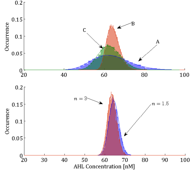
Fig. 5. Steady state distributions for 10,000 cells of AHL concentration in the different architectures of Fig. 1. In the top figure architectures A, B and C are shown. The bottom figure shows, architecture D with n = 1.5 and also with a steeper controller n = 3 .
