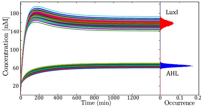
Fig. 4. Time course and steady state histogram of 10,000 cells for architecture D with closed loop with cell to cell communication (with n = 1.5 )
