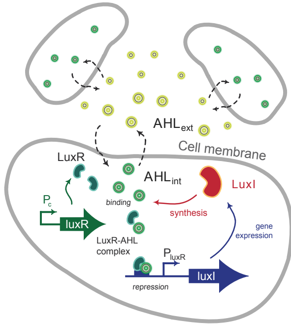
Fig. 2. Schematic of the intracellular feedback control circuit in one cell and the cell-to-cell communication mechanism.
