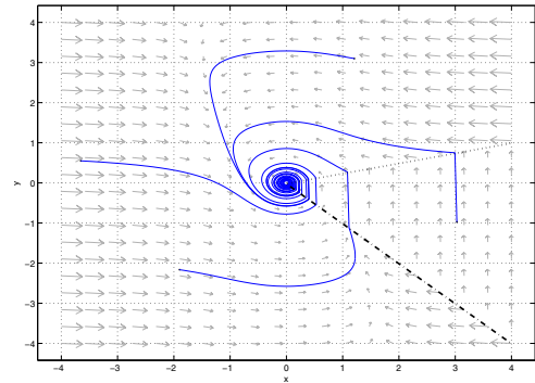
Fig. 3. Trajectories of Hybrid System in Example 2 with p=4 . Dotted line indicates G_{12} and dash-dotted line indicates G_{21}
