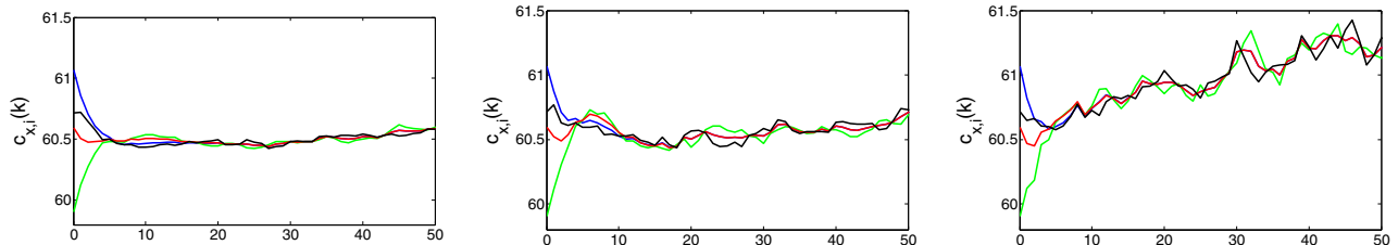
Fig. 6. Evolution of the first component of the centers c_{x,i}(k) applying Algorithm 2 with \varepsilon = 0.5 and \alpha = 0.2 , \alpha = 0.5 and \alpha = 1 respectively.
