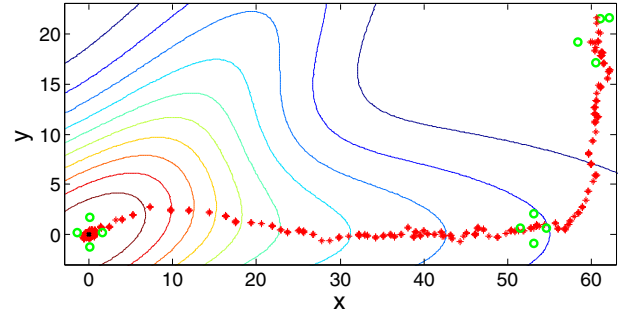
Fig. 5. Source-seeking Algorithm 2 via a circular formation of agents when the measurements are corrupted by Gaussian white noise ( \varepsilon = 0.5 , \alpha = 0.5 )
