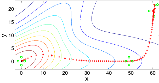
Fig. 2. Source-seeking Algorithm 2 via a circular formation of agents ( \varepsilon = 0.5 , \alpha = 1 )
