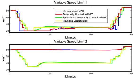
Fig. 3. VSL of segment 3 and 4 for continuous MPC and rounding discretization
