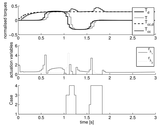
Fig. 6 - Results for the extended linearization controller.
