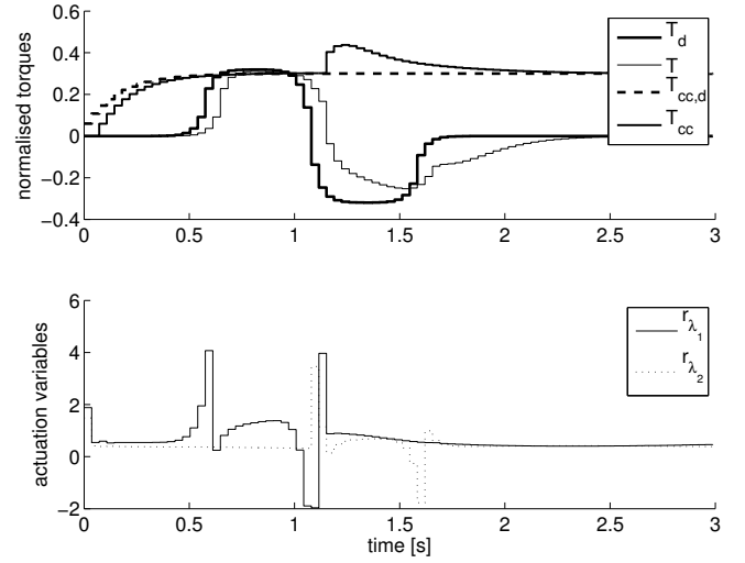
Fig. 5 - Results for the linearization controller without taking constraints on the actuation variables into account. The actuation variables shown in the lower subplot also show the computed negative values. However, for the simulated model the constraints r_{\lambda,i} \geq 0 were applied. Thus, values violating these constraints were set to zero.
