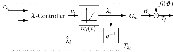
Fig. 2 - The model for one \lambda -Controlled muscle path. Given a reference r_{\lambda_i} for the muscular recruitment \lambda_i , the controller adjusts the stimulation intensity v_i . The nonlinear recruitment function r_{c_i} describes the recruitment. The resulting closed loop T_{\lambda_i} has an approximately linear dynamics. The calcium dynamics G_m models the dependency of the muscular activation \sigma_i on \lambda_i . The muscular torque T_i is then modeled by the multiplication of the angle-dependent function f_i with \sigma_i .
