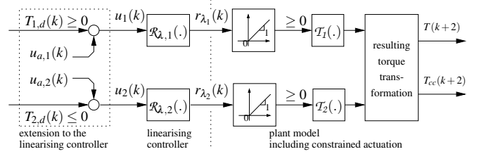
Fig. 4 - An extension is applied to the linearizing controller in the presence of constrained actuation by modification of the signals u_1 and u_2 . The calculated actuation variable of the linearization controller is applied to the plant, which additionally includes the constraints on the actuation variables r_{\lambda_i}(k) .
