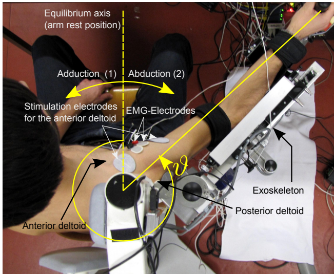
Fig. 1 - Experimental Set-up.
