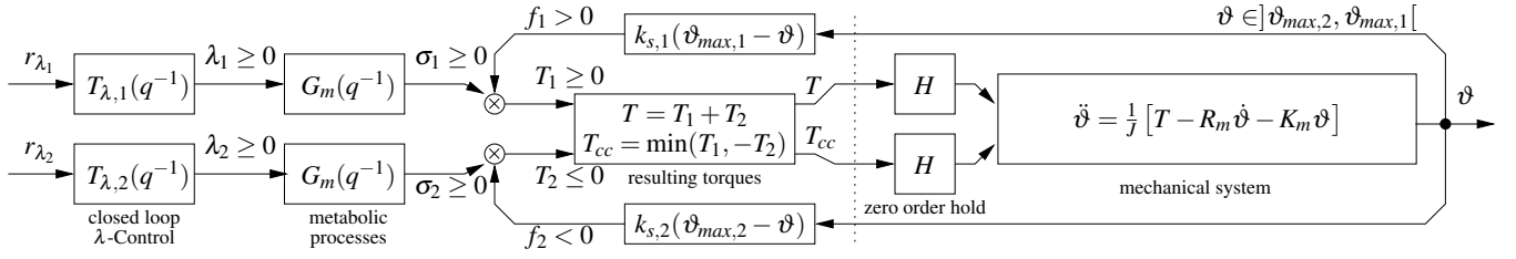
Fig. 3 - Neuro-musculoskeletal model used for controller design.
