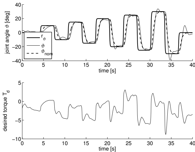
Fig. 7 - Results of a joint-angle control experiment for a healthy subject using the underlying linearization controller with extension and two \lambda -Control loops. The desired co-contraction torque T_{cc,d} was zero.
