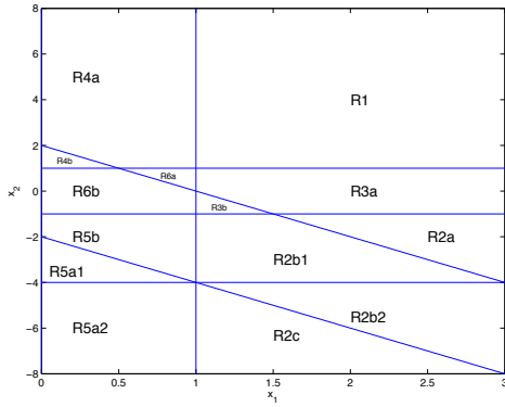
Fig. 3. Part of the partition for \mathbb{R}^2
