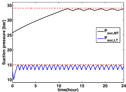
Fig. 5. Suction pressures of two LT and MT sections after applying Algorithm 1.
