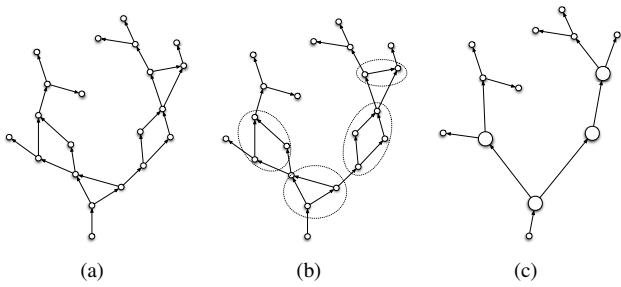
Fig. 4. An example for a rooted cactus network, and augmented systems.
