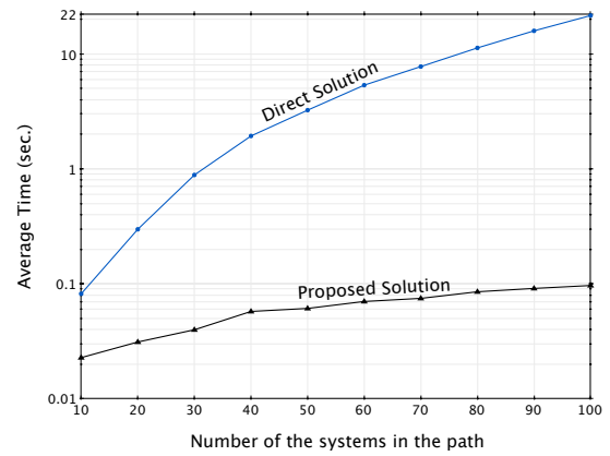
Fig. 6. The average time required to calculate the control inputs for the paths of different lengths using the proposed distributed scheme and the case where the global problem is solved.
