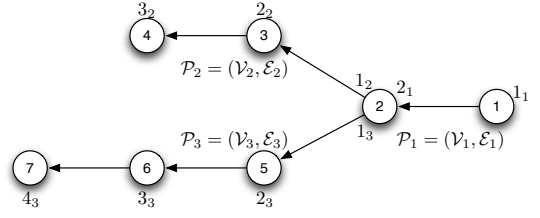
Fig. 3. A sample rooted tree and three paths with vertex sets \mathcal{V}_1 = \{1, 2, 1\} , \mathcal{V}_2 = \{1, 2, 2, 3\} , and \mathcal{V}_3 = \{1, 3, 3, 3, 4, 3\} .
