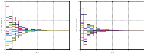
Fig. 5. The trajectories of 20 systems coupled through control inputs.
