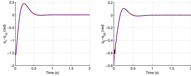
Fig. 4. Error trajectories for the manipulator. Initial conditions [q_m(0) p(0) q_c(0)] = [0 \ 0 \ 0 \ 0 \ 0] . Blue solid lines: a_i = \omega_2 , b_i = 1 , d_i = 284.6 . Red dashed lines: b_i = 10 , d_i = 28.46 . Black dotted lines: b_i = 50 , d_i = 5.69 .
