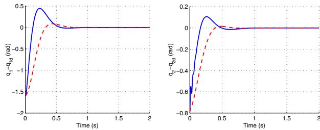
Fig. 5. Error trajectories for the manipulator. Initial conditions [q_m(0) p(0)] = [0 \ 0 \ 0 \ 0] . Blue solid lines: q_c(0) = [0 \ 0] . Red dashed lines: q_c(0) = -B\bar{q}_m(0) .
