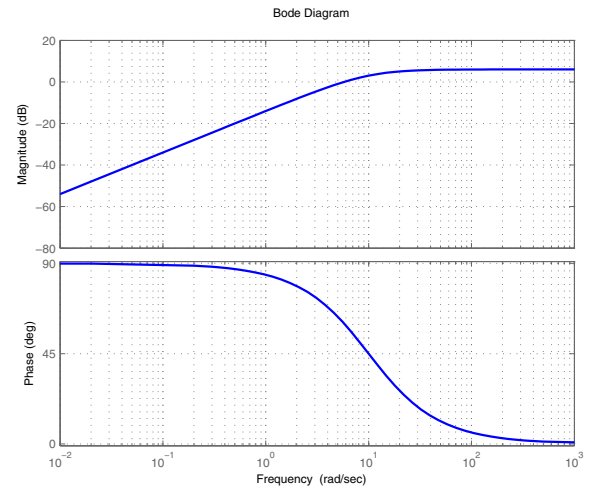
Fig. 1. Bode plot for the tamed differentiator (19) with \kappa_i = 2 and \rho_i = 10 .
