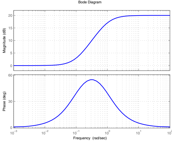
Fig. 2. Bode plot for the lead-compensator (20) with \omega_1 = 0.1 and \omega_2 = 1 rad/s.
