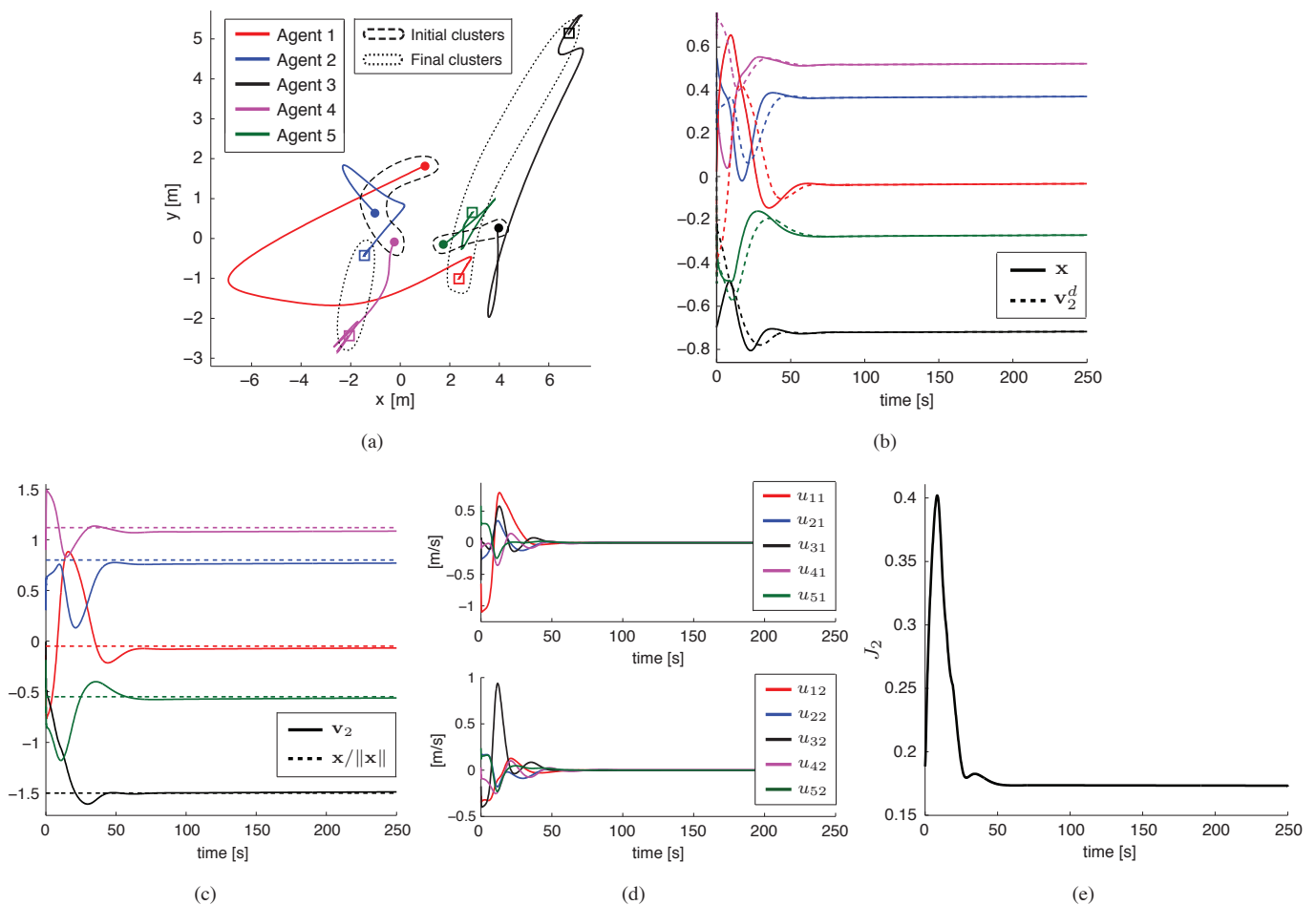
Fig. 2. Clustering control : (a) Trajectory of the 5 agents (the initial and final positions are marked with bullets and squares, respectively); the initial and final clusters are indicated with dashed and dotted sets, respectively; (b) Time history of the estimated Fiedler vector \mathbf{x} (solid) and \mathbf{v}_2^d (dash); (c) Time evolution of normalized \mathbf{v}_2 (solid) and of \mathbf{x}/\|\mathbf{x}\| (dash); (d) Time history of the control inputs \mathbf{u}_i = [u_{i1}, u_{i2}]^T , i \in \{1, \dots, 5\} ; (e) Time evolution of the cost function J_2 . Note that in (b) and (c) we used the same colors' convention as in (a) and (d).
