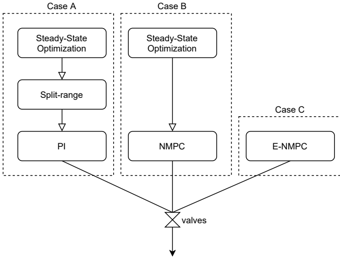
Fig. 1. Control structures
