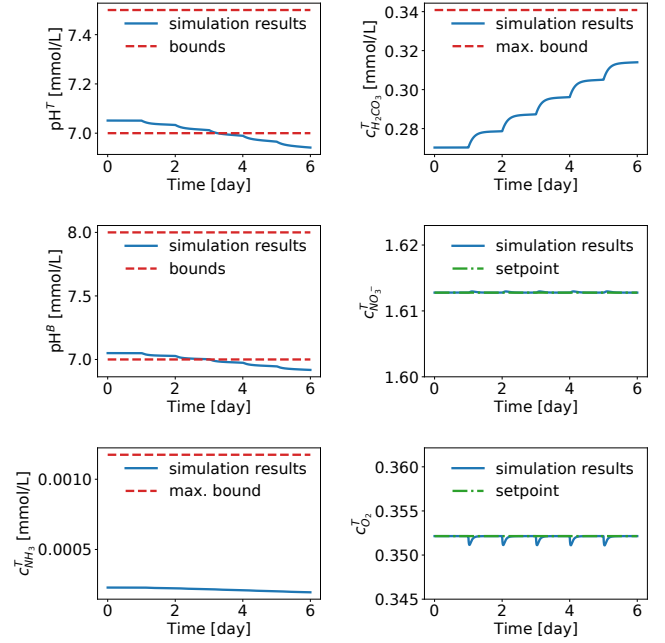
Fig. 3. Dynamic behavior of the process with oxygen and nitrate controls, and subjected to disturbance, F
