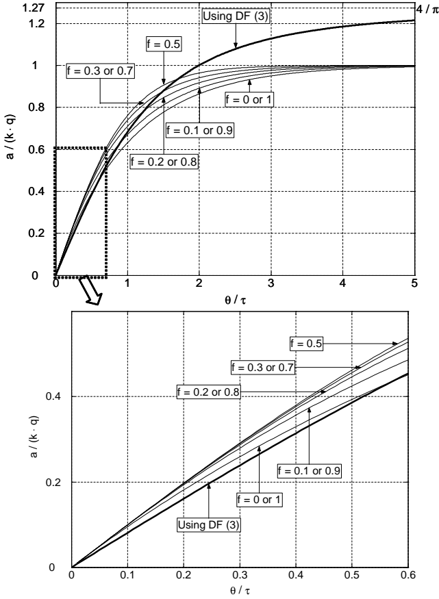
Fig. 6. The amplitude in (15) agrees surprisingly well with the describing function analysis (11) provided \theta/\tau is small.
