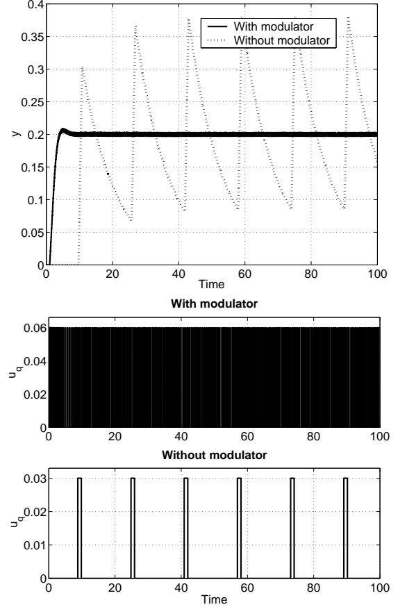
Fig. 7. Simulation results for the system given by (13) and (14) using a modulator ( r_0 = 0.2 ).
