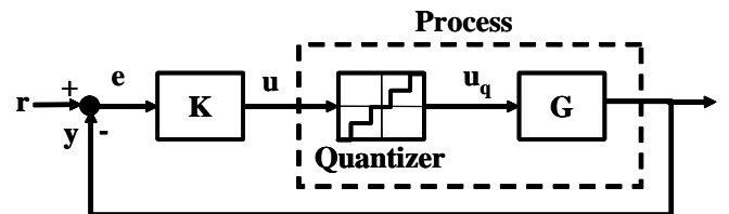
Fig. 1. Feedback control configuration for the valve inaccuracy problem.
