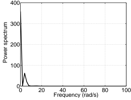
Fig. 4. Power spectrum of the limit cycle of the system described by (6) and (7) for q = 1 .
