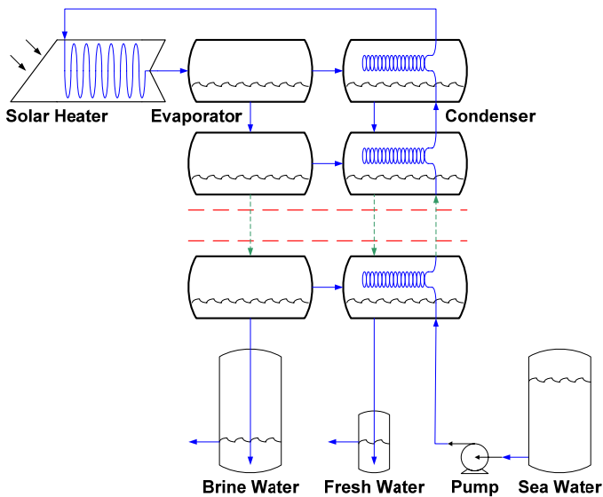
4. Multi-stage configuration of the proposed system
