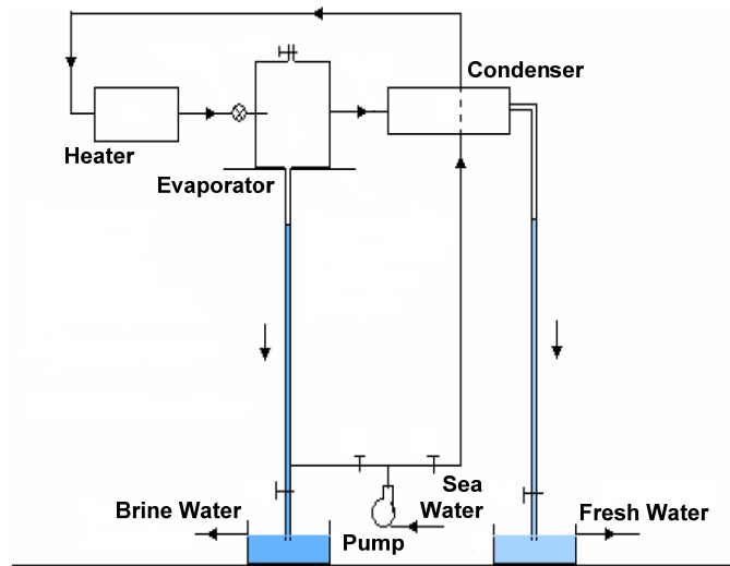
2. Passive vacuum flash desalination system
