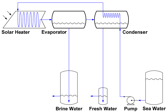
3. Proposed desalination system
