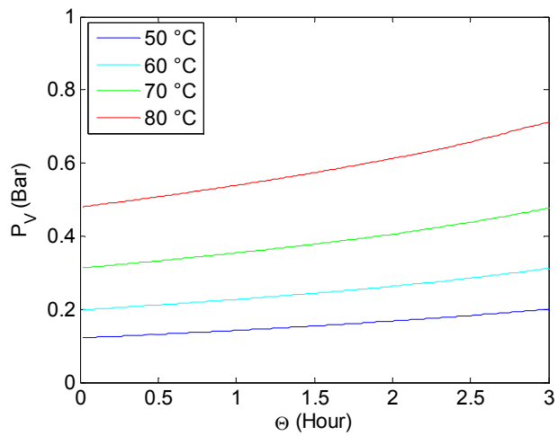
8. Vacuum pressure at several flash temperatures
