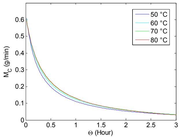
9. Production rate at several flash temperatures
