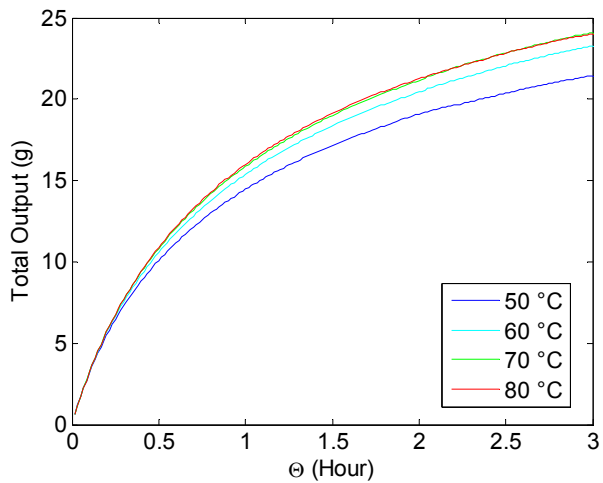
10. Production amount at several flash temperatures
