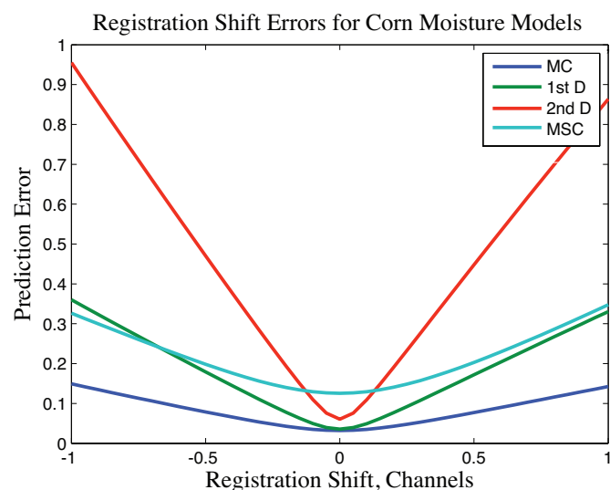
Figure 5. Model prediction error as a function of registration shift for models with mean centering, first derivative, second derivative and multiplicative scatter correction.
