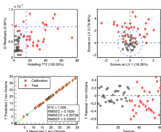
Figure 2. Calibration Model applied to high T^2 data. Individual plots as in Figure 1.
