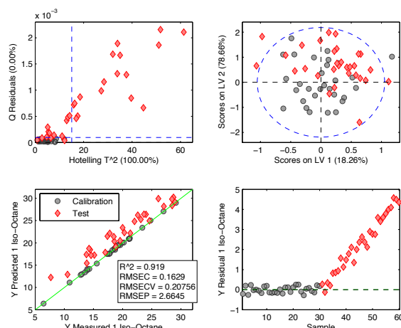
Figure 3. Calibration model applied to data with progressively high Q values. Individual plots as in Figure 1.
