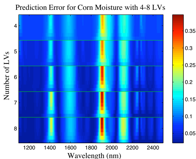
Figure 6. Model prediction error as a function of interferent peak width, peak location, and number of model LVs.
