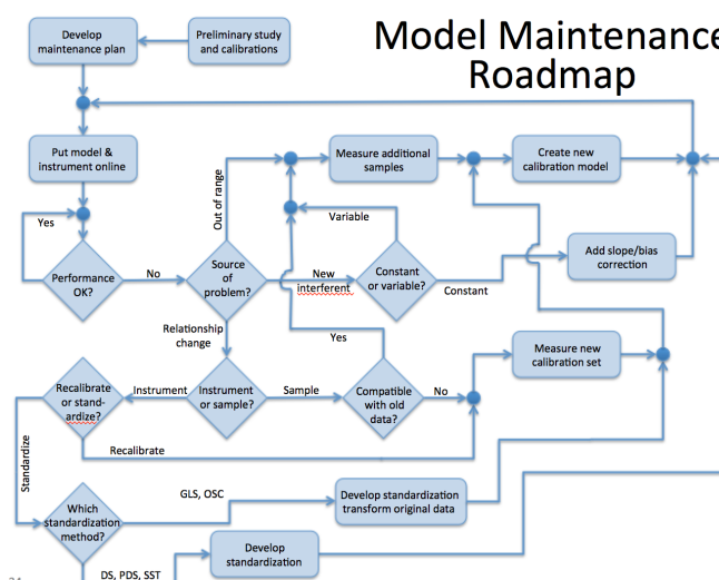
Figure 4. Model maintenance roadmap flowchart
