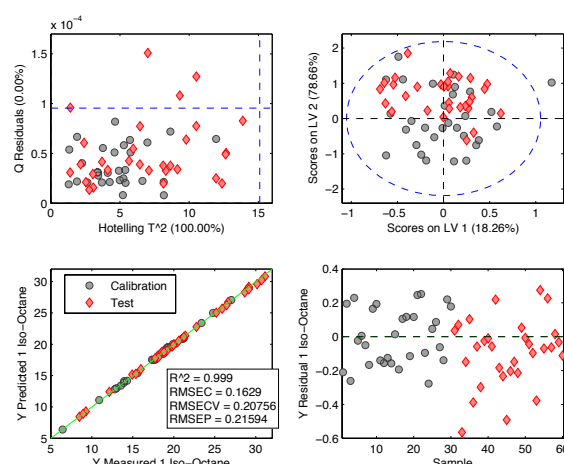
Figure 1. Calibration model applied to “normal” data including Q versus T^2 (upper left), scores on first two latent variables (upper right), predicted versus actual values for iso-octane (lower left) and prediction residual versus sample number (lower right). In all plots the calibration data is shown as grey circles while the test data is shown as red diamonds.
