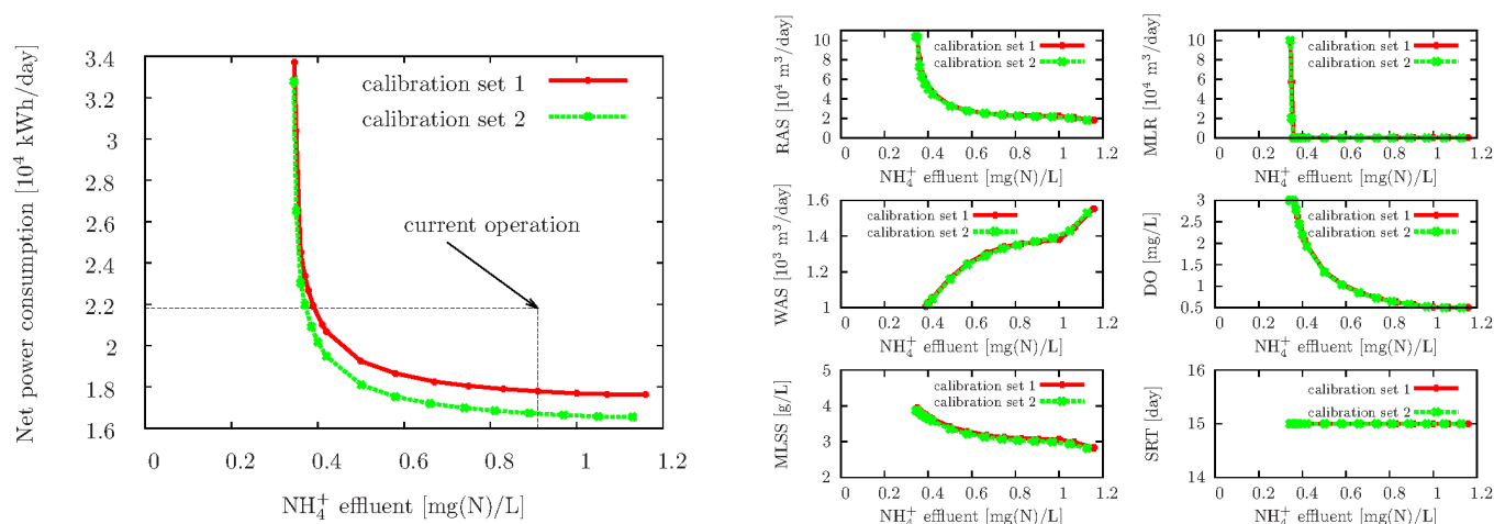
Fig. 3. Effect of ammonia discharge level on the net power consumption (left plot) and on the decision/operational variables (right plots), for the two calibration sets in Table 3.
