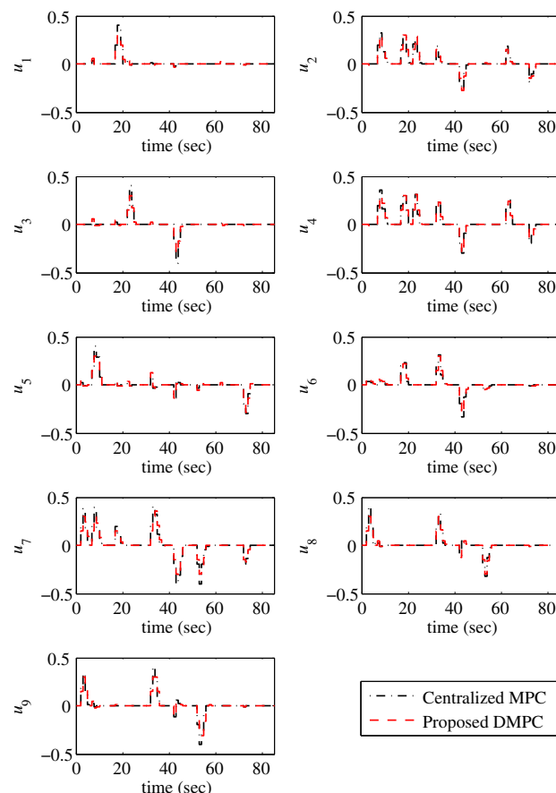
Fig. 3. The evolution of the inputs under the centralized MPC, and N-step Impacted-region optimization based DMPC.
