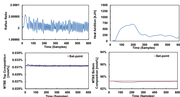
Fig. 7. Closed-loop performance of the control structure for Design (I) to a disturbance in the feed.
