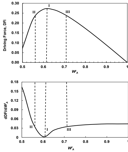
Fig. 4. Driving force diagram for W_A – W_B separation (reactive zone only – top figure) and its corresponding derivative of DF_i with respect to W_A^I (bottom figure).
