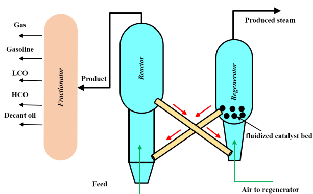
Fig. 3. A flow diagram of a Fluid Catalytic Cracking unit
