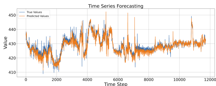
Fig. 4. The performance of Informer soft sensor on test data
