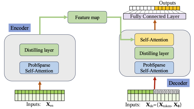
Fig. 1. Informer model overview
