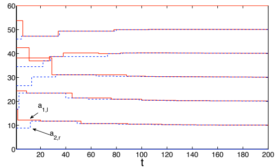
Fig. 3. Behavior of the extremes when aOPA is applied with N = 6 cameras.
