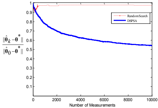
Fig. 5. Performance of localized random search method and DSPSA with noisy measurements for skewed quartic function.
