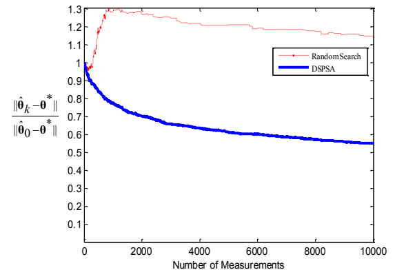
Fig. 4. Performance of localized random search method and DSPSA under noise-free situation for skewed quartic function.
