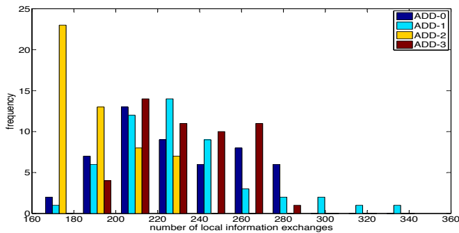
Fig. 2. Histogram of the number of local communications required to reach \|g(\lambda_k)\| \leq 10^{-10} for ADD- N with respect to parameter N , for 50 trials of the network optimization problem on random graphs with 25 nodes and 75 edges. ADD-2 is shown to be the best on average by about 10% indicating that with respect to communication cost, larger N is not necessarily better.
