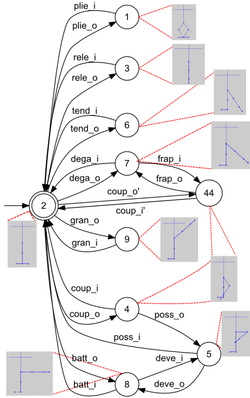
Fig. 2. A discrete event model of the working leg of a dancer during a ballet barre exercise. States correspond to poses defined by three joint angles: hip, knee, and ankle. Events are given by primary ballet movements plus the empty event (or hold), which corresponds to undrawn self-loops. Images of the poses and corresponding states are shown for clarity. Here it is clear that, in our model, state 44 is physically the same as state 4. We differentiate these two related states based on whether the motion of the leg is to remain low (below the hips) or high (at or above hip level) before returning to a neutral state and beginning the next movement. These levels generally correspond to specific movements which stem from two variants of this pose: one where the foot is wrapped around the ankle and one where the foot is fully pointed and placed next to the ankle, as described in [19].
