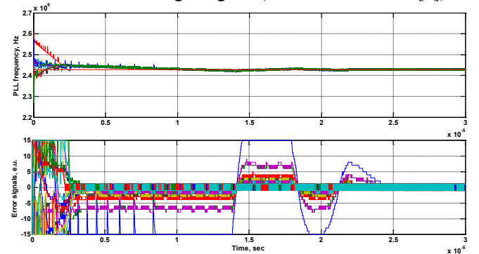
Fig. 6. Simulation results of the 4 \times 4 ADPLL network, upper figure represents the evolution of node frequencies, bottom - the evolution of its relative phase error signal. Each PLL node is presented with a unique color.
