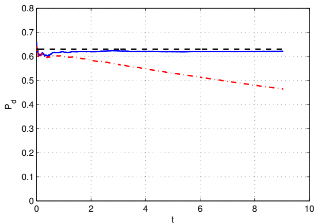
Fig. 6. Event detection probability P_d vs time t for decaying networks with given P_{des} = 0.63 (constant dashed line); with scheduling scheme (solid line) and without scheduling scheme (decaying dashed line). Here \lambda = 10 , A(0) = 1 , \gamma = 1 and c = 1 .
