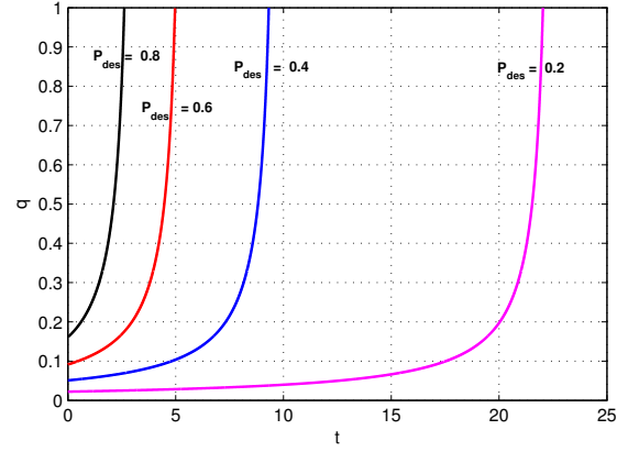
Fig. 1. Evolution of probability of a sensor being on for a given desired performance P_{des} where \lambda = 10 , c = 1 and r = 2 . In each case, lifetime of the network is achieved when q = 1 .
