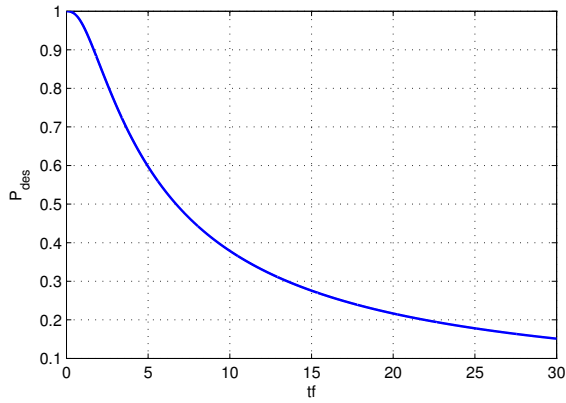
Fig. 2. Lifetime t_f of network vs desired network performance P_{des} . The parameters are \lambda = 10 , c = 1 and r(0) = 2 .
