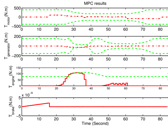
Fig. 6. MPC results: Engine, motor, and generator's torque and constraints
