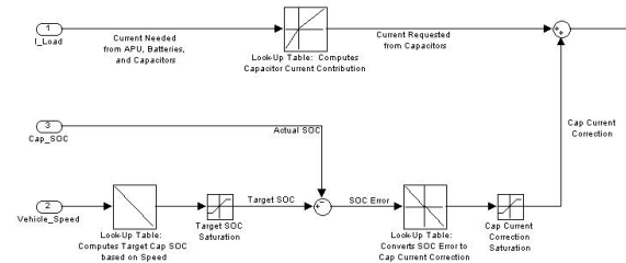
Fig. 6. The feedforward and feedback control structure used to determine a reference current for the inductor current controller.
