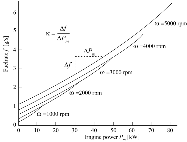
Fig. 2. Characteristic fuel map of an SI-engine
