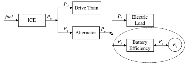
Fig. 1. Block diagram of vehicle's power flow
