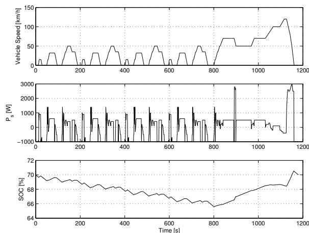
Fig. 4. Simulation results for P_l = 1000 W
