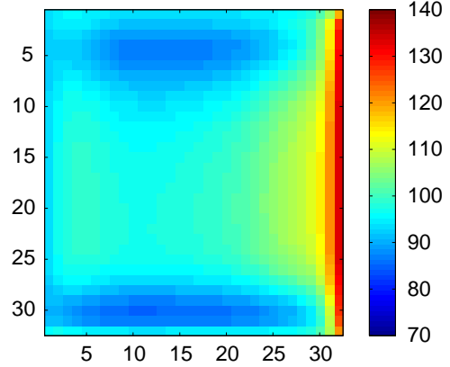
Fig. 1. Simulated heated plate example. The plate is heated or cooled along the complete edges on all sides. The physical equation are solved on a 32 by 32 grid in 5 Euler integration steps.
