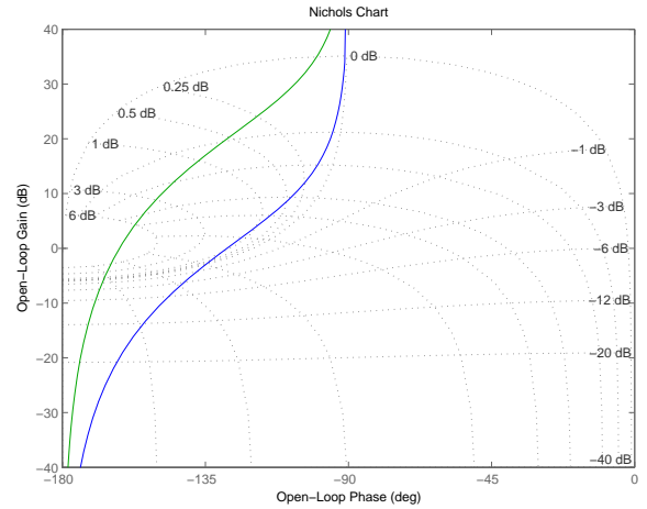
Fig. 5. Nichols chart for L_1(s) and L_2(s) . The change in gain between L_1(s) and L_2(s) corresponds to a shift up the vertical axis. Since L_2(j\omega) approaches closer to the s = -1 point, the closed-loop frequency response will appear much higher up the “foothills” of Mount Nichols.
