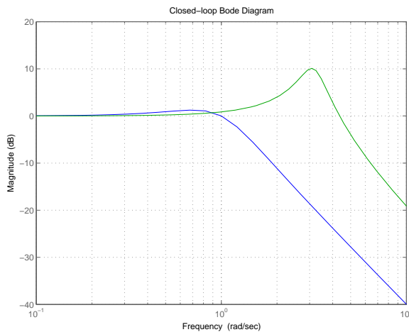
Fig. 12. Closed-loop Bode plot for L_1(s) and L_2(s) . The 10-dB peaking in the response agrees with the 10-dB contour in Figure 11 and the associated height on the foothills of Mount Hall.
