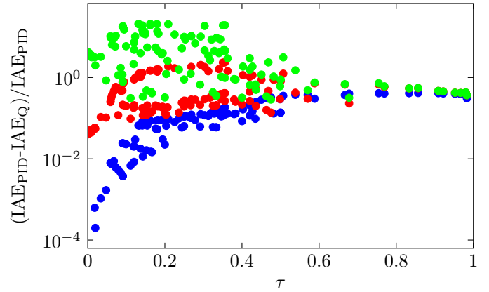
Fig. 6. Relative IAE improvement of Q over IAE design, for M_{ks} = 1 (blue), M_{ks} = 10 (red), and M_{ks} = \infty (green), plotted against normalized time delay, \tau , for the processes considered in Section 3.2.
