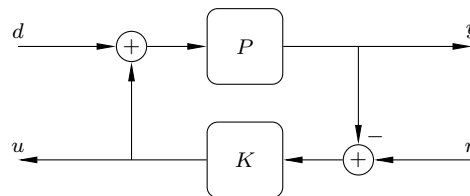
Fig. 1. Closed-loop control system with process P , controller K , process output y , load disturbance d , control signal u , and measurement noise n .
