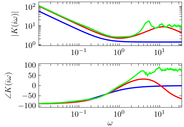
Fig. 3. Controller Bode plots. Controllers and colors as in Figure 2.
