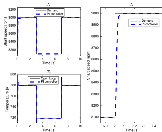
Fig. 7. Variation of the simulated measurements with respect to time from MATLAB/Simulink model of Case Study 3.
