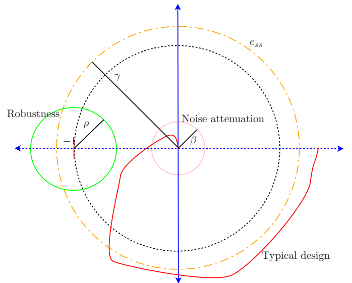
Figure 3. Open-loop transfer function, L(s) , specifications in the Nyquist diagram.
