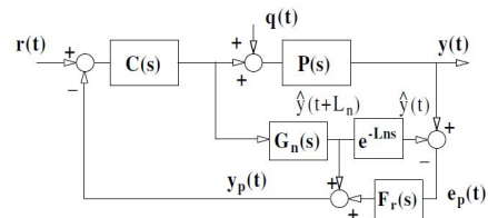
Fig. 3. Filtered Smith Predictor control structure (Normey-Rico and Camacho, 2007).
