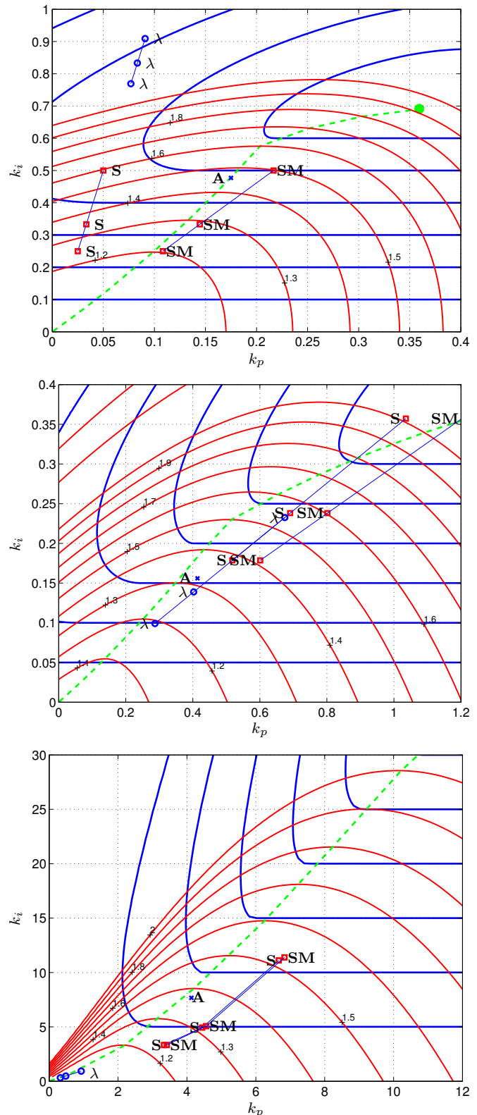
Fig. 2. Scaled trade-off plots with controller parameters obtained with a the tuning rules: lambda tuning ( \lambda ), SIMC (S), modified SIMC (SM) and AMIGO (A). The plot shows from top to bottom systems with delay dominated, balanced and lag-dominated dynamics. The dashed lines are the loci of controller gains that minimize IAE for a given robustness.
