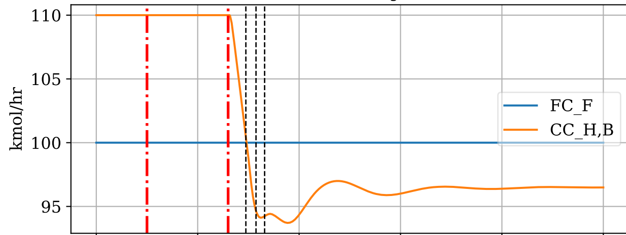
Select Min Feed Rate ( \Delta y_S^* = 10 kmol/hr)
