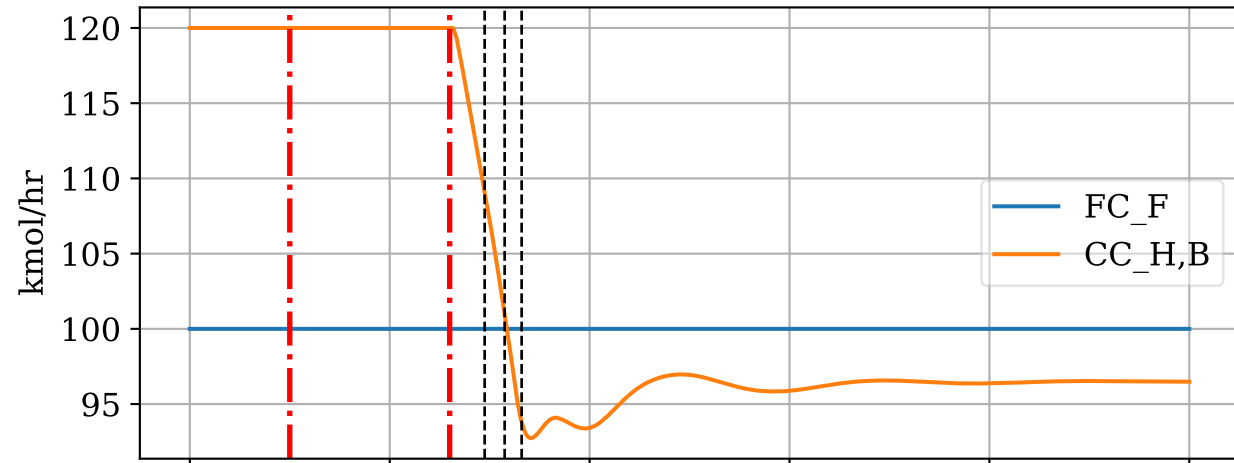
Select Min Feed Rate ( \Delta y_S^* = 30 kmol/hr)
