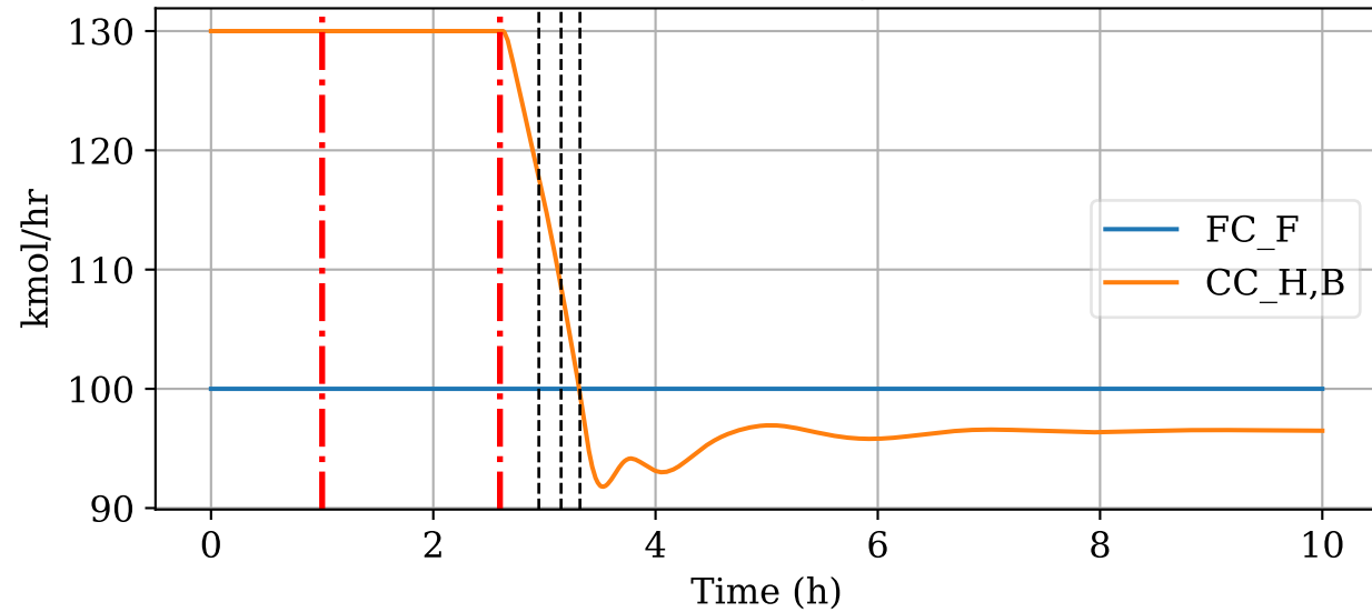
Select Min Feed Rate ( \Delta y_S^* = 30 kmol/hr)
