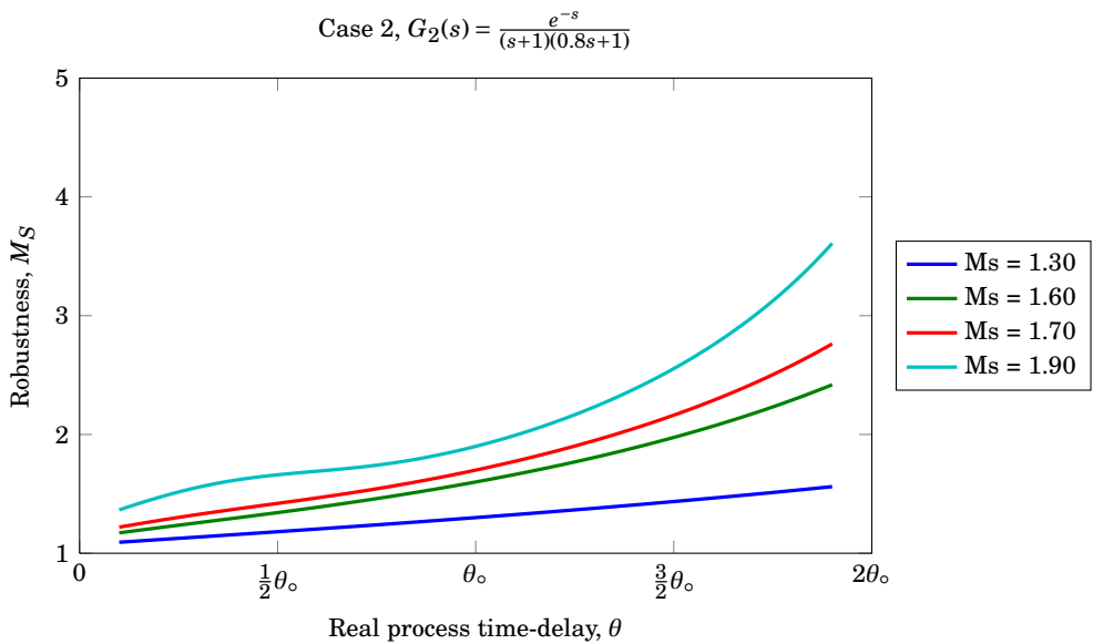
Figure E.2 – Performance and robustness sensitivity to modelling error in the time-delay parameter for a Pareto optimal Smith predictor PI controller for a set of target M_S values for model G_2(s) = \frac{e^{-s}}{(s+1)(0.8s+1)} .
