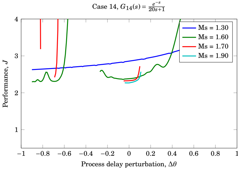
(a) Performance sensitivity, J = f(\theta) .
