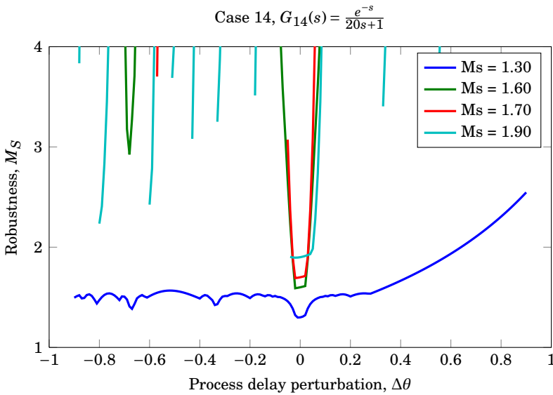
(b) Robustness sensitivity, M_S = f(\theta) .
