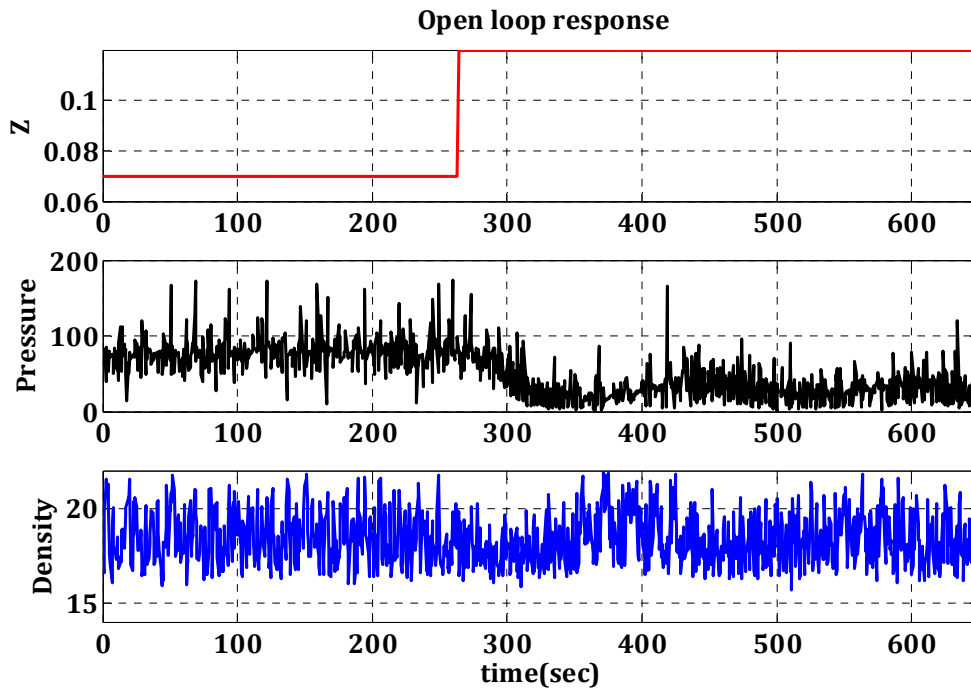
Figure 5.16: Open-loop step response of conductance probe (density meter) in the stable region. The first plot ( Z ) shows the step change in valve opening, the second plot presents the step response of top pressure in Kilo Pascal and the third plot illustrates the step response of the outflow density in kg/sec.
