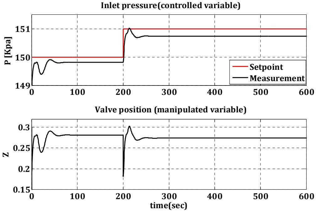
Figure 5.24: Set-point step change using initial choke valve opening of 30% and the initial gain of K_{c0} = 0.1 . An overshoot of D=0.3 , as the recommended value by Shams has been achieved.
