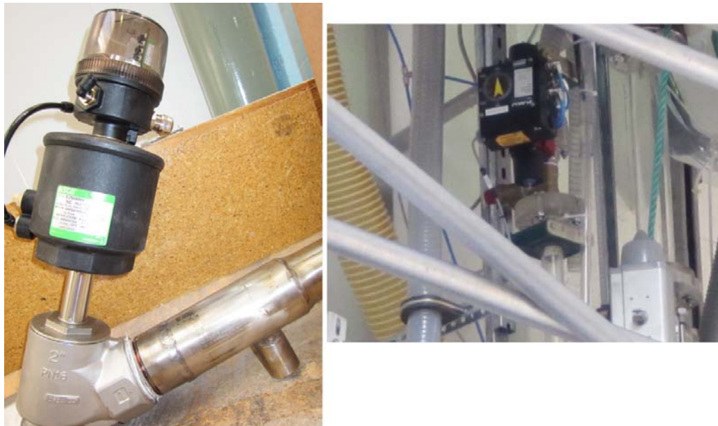
Figure 3.13: Choke valves; left: Fast valve, Right: Slow valve and its positioner
