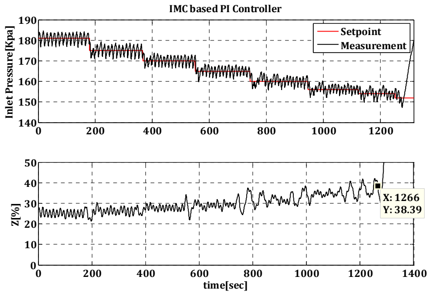
Figure 5.7: Result of control using the IMC-based PI controller. The controller has been able to move the bifurcation point from Z=26\% up to Z=38.39\% .
