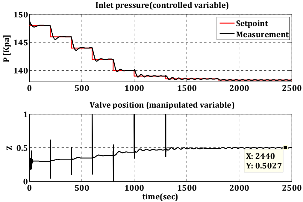
Figure 5.29: Simulation result of control using the IMC-based PID controller tuned at the initial choke valve position of 30%.
