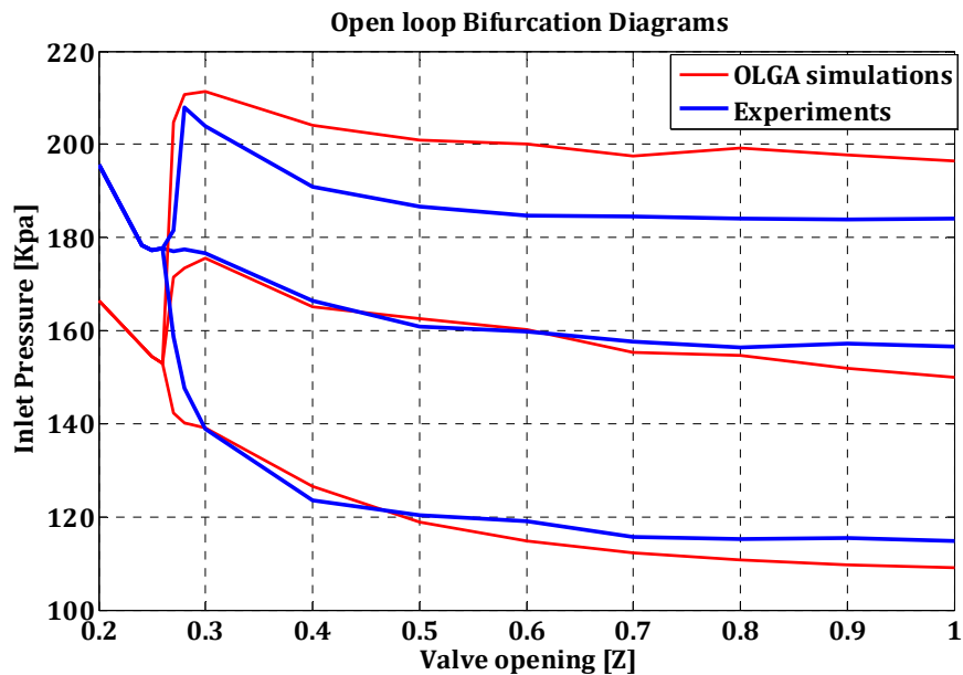
Figure 5.37: simulated results from the OLGA case compared with the experimental results from valve1. The bifurcation point is fairly the same for both models.
