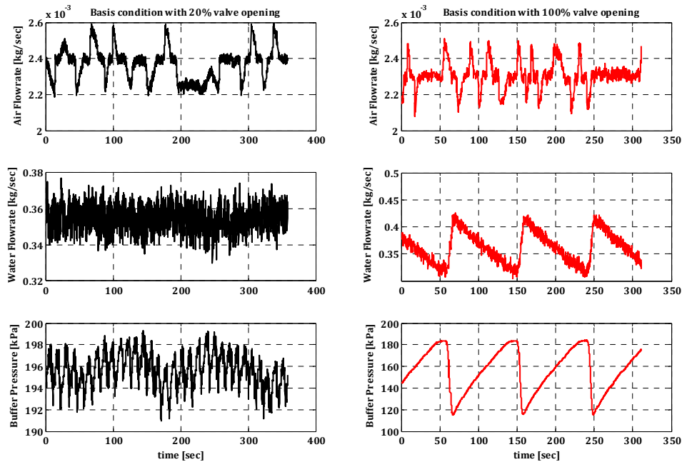
Figure 5.1: Illustration of basis open-loop conditions in case of flow rates and pressure. The left series of plots are illustrating the system with valve opening Z=0.2 that is related to the stable region while the right side plots present the system with valve opening Z=1 that is related to the unstable region. Large oscillations are clear signs of instability at Z=1 .
