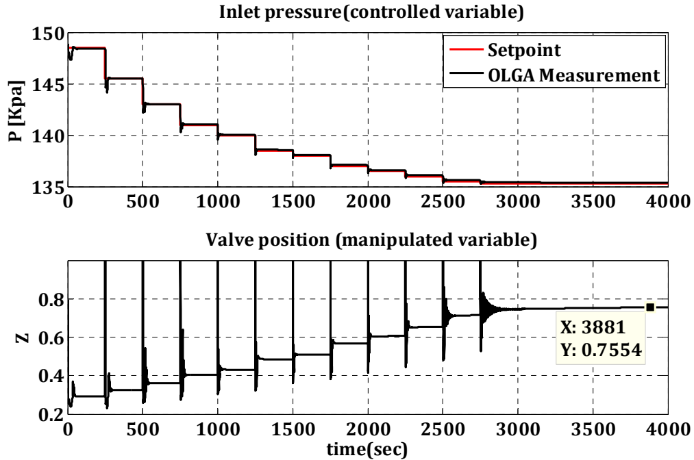
Figure 5.35: Simulation result of control using gain scheduling between PI controllers tuned for the initial choke valve position of Z=30\% .
