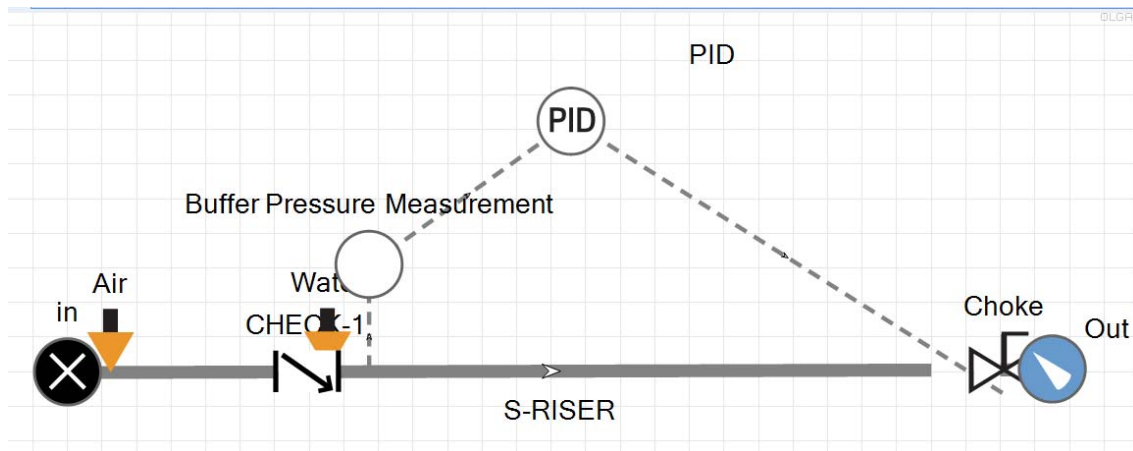
Figure 4.2: OLGA case with PID controller. The controller receives the measurement signal from the pressure transmitter and sends the output signal into the choke valve located at top of the riser.
