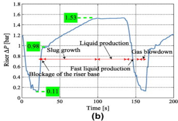
Figure 2.7: Stages for SS1 (a) a graphical illustration (b) marked on a cycle of an experimental riser \Delta P trace ( U_{SL} = 0.20\text{ms}^{-1} and U_{SGO} = 1.00\text{ms}^{-1} ) (Malekzadeh, Henkes et al. 2012)
