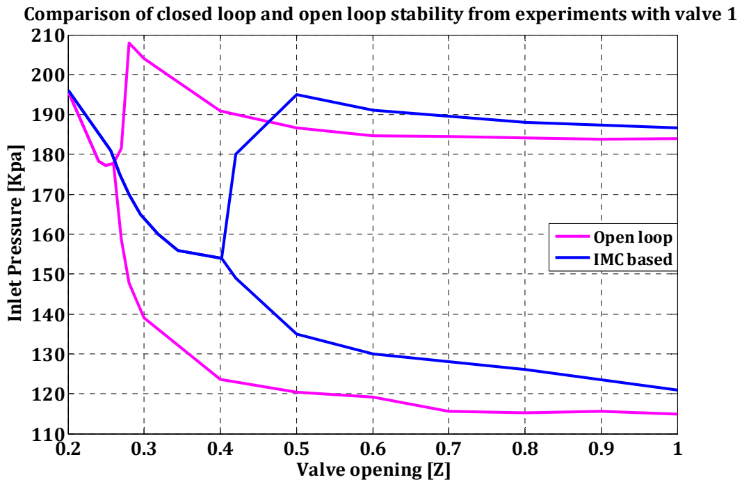
Figure 5.39: Comparison between the stabilizing control results from IMC-based tuning method and the open-loop system for the experiments with valve 1.
