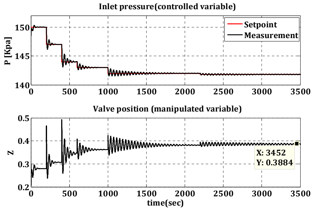
Figure 5.25: Simulation result of control by Shams's closed-loop method for the initial choke valve position of 30%. The values of Z=0.389 and P=142 kpa have been the maximum achieved valve opening and the minimum achieved set-point, respectively.
