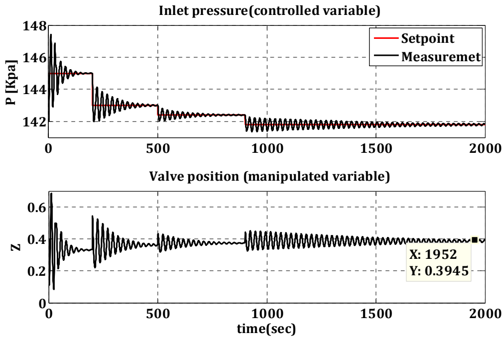
Figure 5.27: Simulation result of control by Shams's method for the initial choke valve position of 40%. The values of Z=0.395 and P=142 kpa have been the maximum achieved valve opening and the minimum achieved set-point, respectively.
