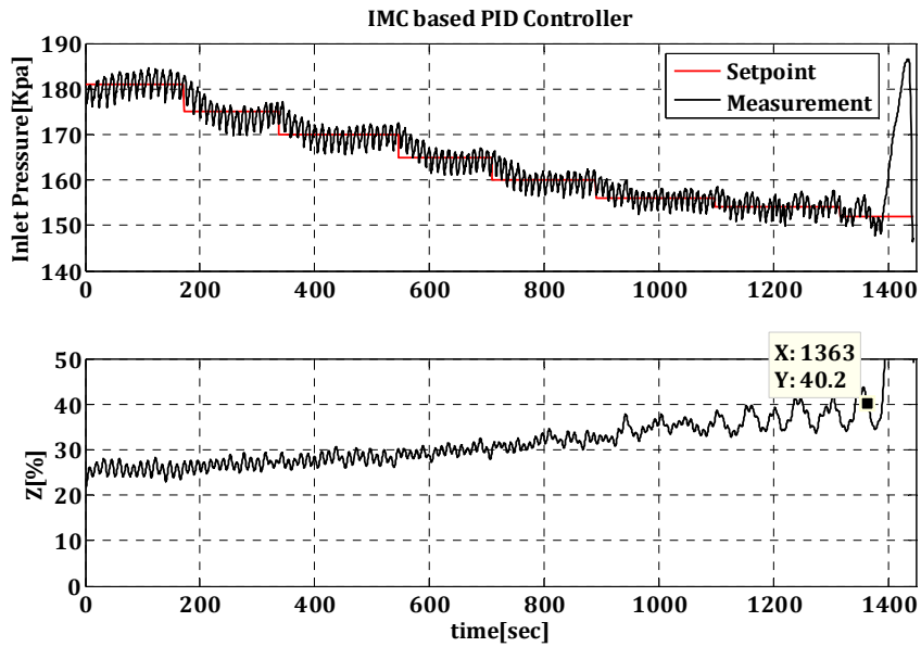
Figure 5.6: Result of control using the IMC-based PID controller. The controller has been able to move the bifurcation point from Z=26\% up to Z=40.2\% .
