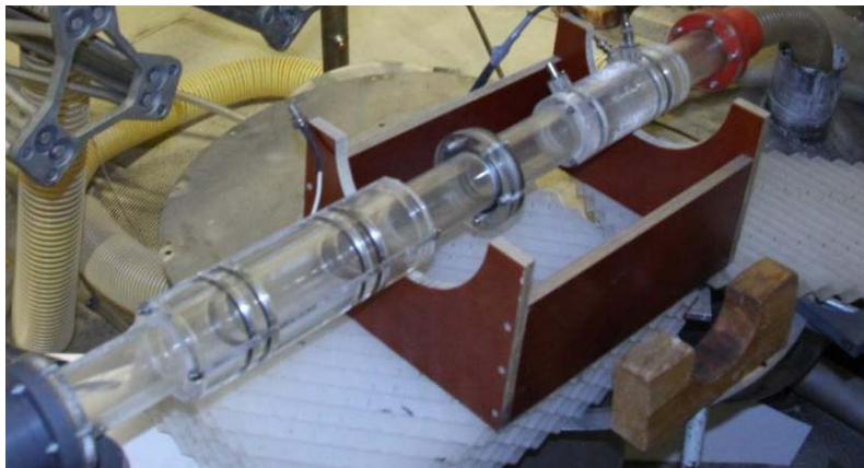
Figure 3.14: The conductance probe
