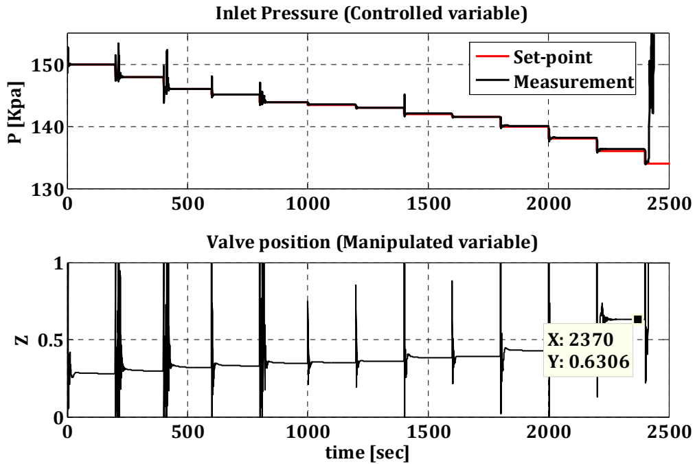
Figure 5.22: Simulation result of control by P-Only controller for K_c = 1
