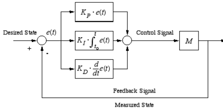
Figure 2.9: A typical PID control structure
