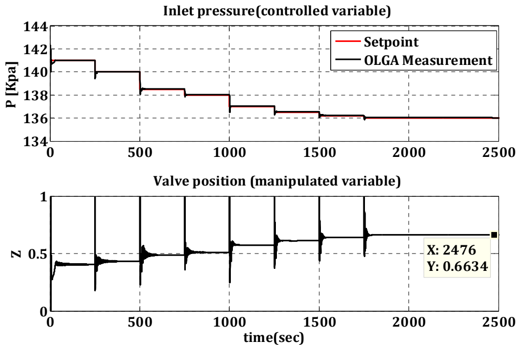
Figure 5.36: Simulation result of control using gain scheduling between PI controllers tuned for the initial choke valve position of Z = 40%.
