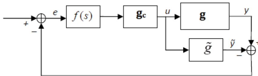
Figure 2.11: The internal model control (IMC) structure
