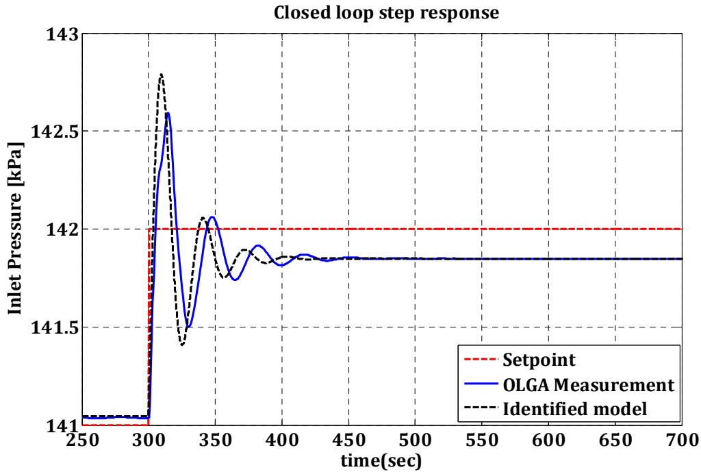
Figure 5.31: Closed-loop response of step change at initial valve opening Z=0.4. The dashed black line shows the transfer function of the IMC-based identified model.
