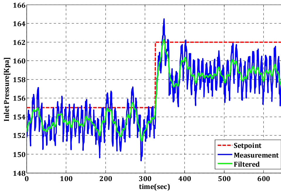
Figure 5.9: Set-point step change for a closed-loop feedback experiment with a P_only controller using inlet (buffer) pressure as control variable. A low pass filter with a smoothing factor of \alpha = 0.25 was used to remove the noise effect from the response.
