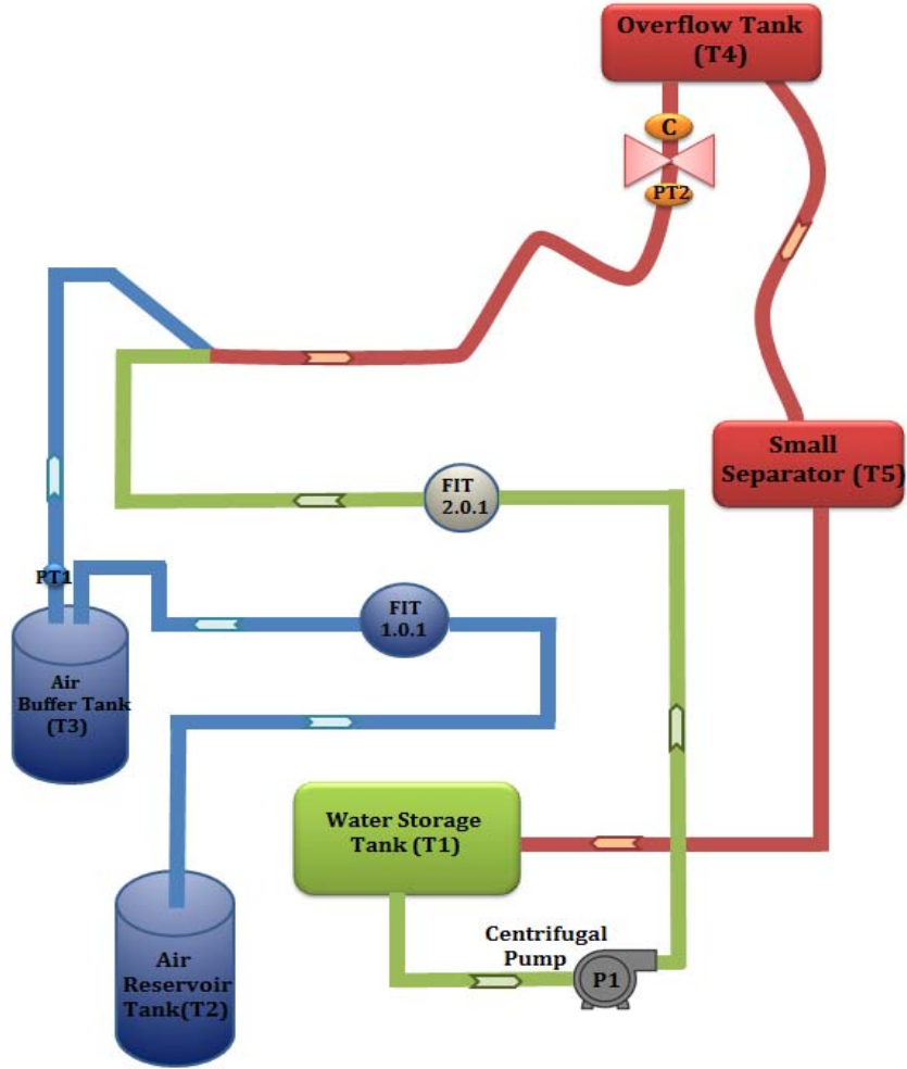
Figure 3.3: Medium scale Test Rig Layout with more details, NTNU
