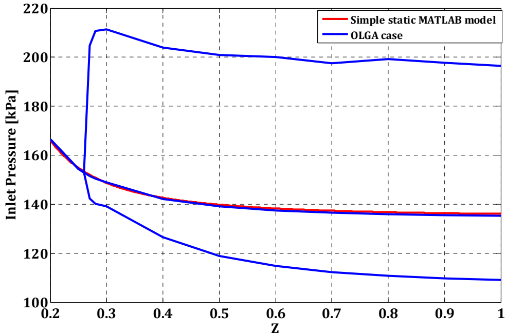
Figure 5.34: Simple static MATLAB model compared to the OLGA model. The blue midline in the figure presents the steady state values of the inlet pressure from OLGA simulations and the red midline is the values of inlet pressure from the MATLAB model. The top and bottom blue lines show the maximum and minimum values of pressure oscillations at each operating point in the open-loop system.
