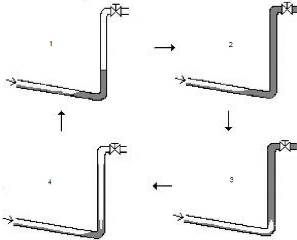
Figure 2.6: Graphical illustration of a slug cycle (Yan and Che 2011). Slug formation is shown in part 1. Slug production is shown in part 2, Blowout in part 3 and liquid fall back in part 4.
