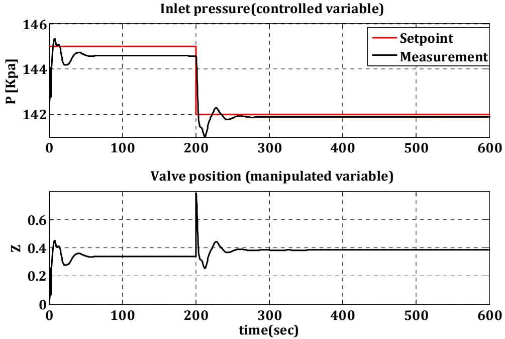
Figure 5.26: Set-point change using initial choke valve opening of 40% and the initial gain of K_{c0} = 0.15 . An overshoot of D=0.32 , near to the recommended value by Shams has been achieved.
