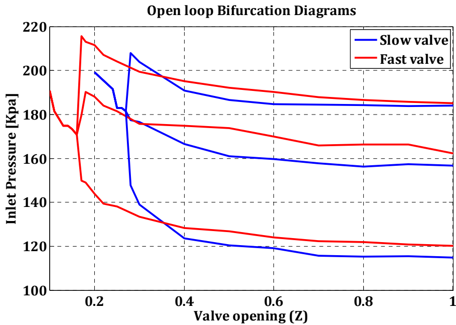
Figure 5.18: Comparison of inlet pressure between the slow valve and the fast valve at their different operating points for the open-loop system. At a certain level of valve opening, the slow valve gives a lower inlet pressure.
