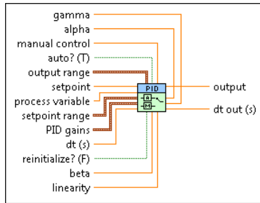
Figure A.1: PID Advanced (DBL)
