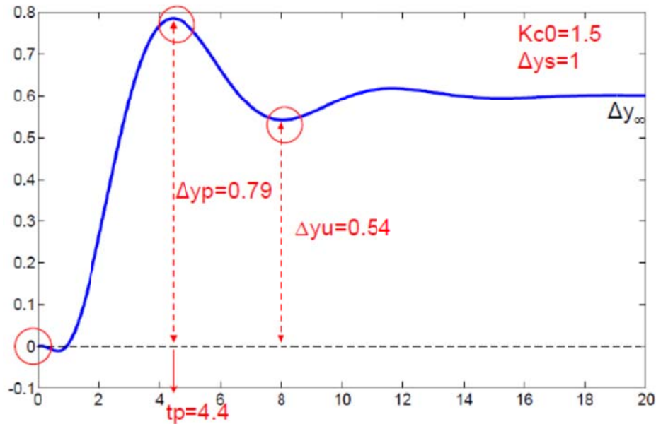
Figure 2.10: closed-loop set-point response with P-only controller (Skogestad and Grimholt 2011)
