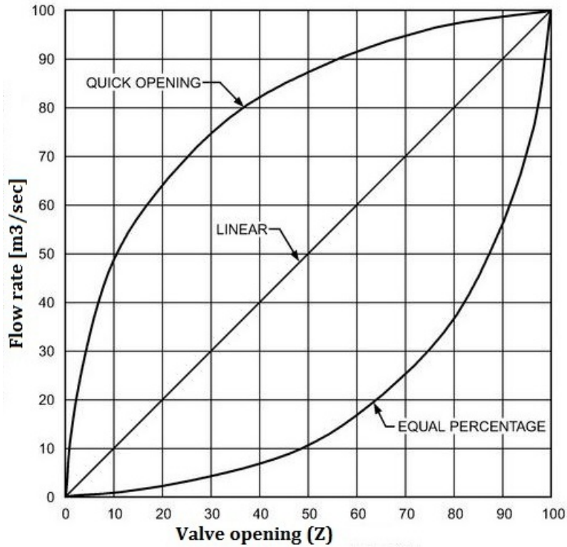
Figure 5.17: Characteristic curves for slow (linear) and fast (quick opening) valves. There is a lower level of valve opening for the fast valve at a specific flow rate (for instance 50), meaning that the fast valve can produce the same flow rate as the slow valve even at lower levels of valve opening.
