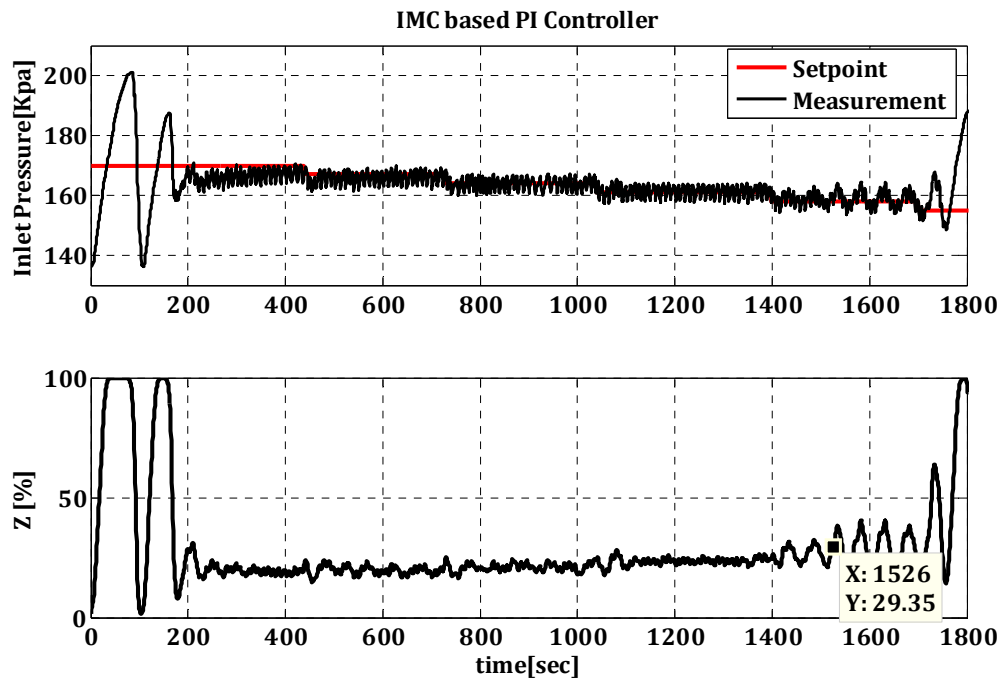
Figure 5.12: Result of control using the IMC-based PI controller. The controller has been able to move the bifurcation point from Z=16\% up to Z=29.35\% .
