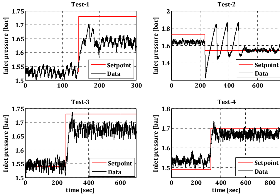
Figure 5.3: Presentation of different tests of set-point step change for a closed-loop feedback experiment with a P_only controller using inlet (buffer) pressure as control variable. Test-4 shows the best characteristics in case of desired overshoot and steady state gain required for tuning the controller.
