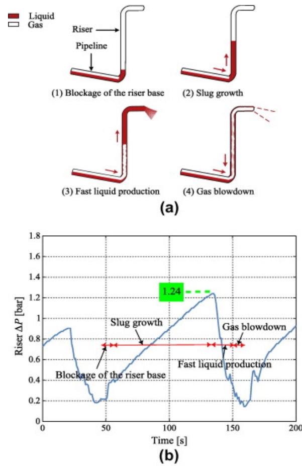
Figure 2.8: Stages for SS2 (a) a graphical illustration (b) marked on a cycle of an experimental riser \Delta P trace ( U_{SL} = 0.10\text{m s}^{-1} and U_{SGO} = 2.00\text{m s}^{-1} ) (Malekzadeh, Henkes et al. 2012)
