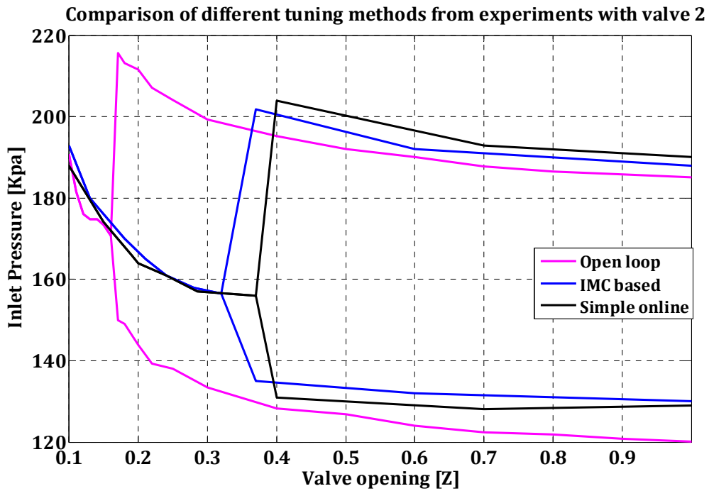
Figure 5.40: Comparison of stabilizing control results from different tuning methods applied in the experiments with valve 2. Simple online method with gain scheduling shows the best performance.
