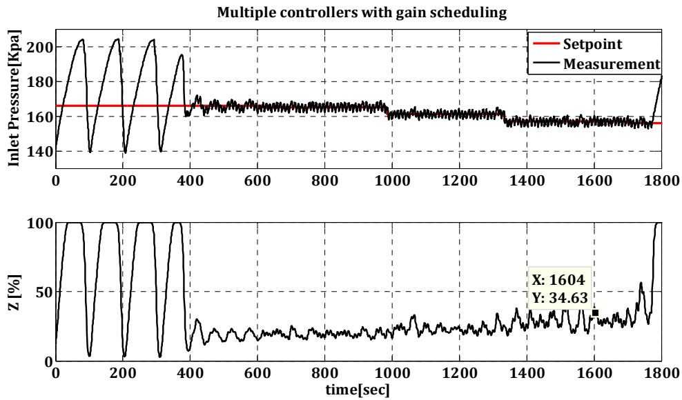
Figure 5.14: Results of gain scheduling using four PI controllers. When the system was switched into the fifth controller the instability was appeared; meaning that the maximum level of stability was reached with four controllers tuned by simple online tuning rules. The controllers have been able to move the bifurcation point from Z=16\% up to Z=35\% .
