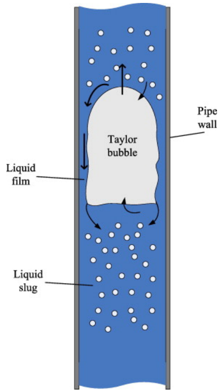
Figure 2.4: Schematic map of slug flow in a vertical pipe in a slug unit (Yan and Che 2011)
