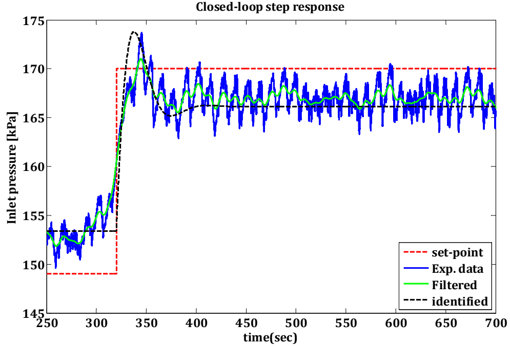
Figure 5.5: Presentation of identified closed-loop step response. The dashed black line shows the identified closed-loop transfer function obtained from IMC design.
