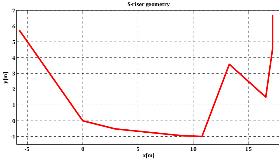
Figure 4.1: Geometry of S-riser in OLGA
