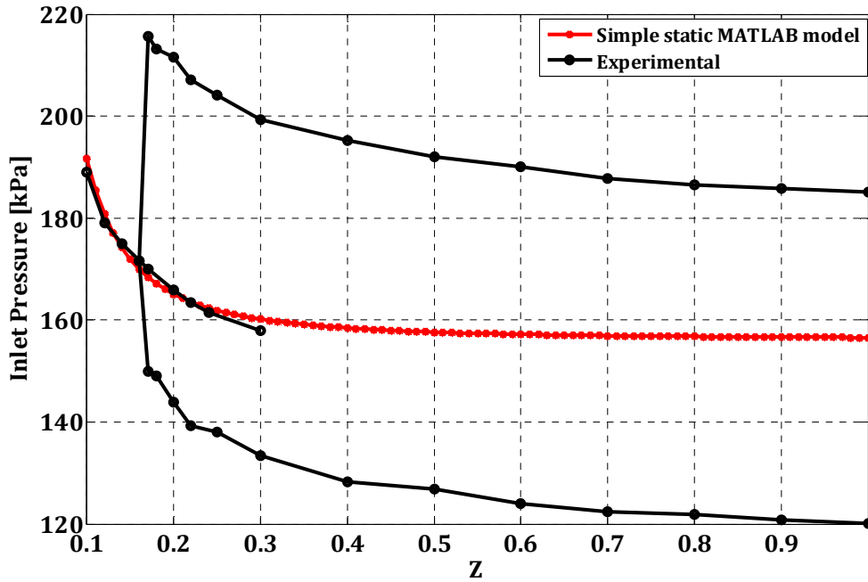
Figure 5.13: Simple static MATLAB model compared to the experimental model. The black midline in the figure presents the steady state values of the inlet pressure and the red midline is the values of inlet pressure from the MATLAB model. The top and bottom black lines show the maximum and minimum values of pressure oscillations at each operating point in the open-loop system.
