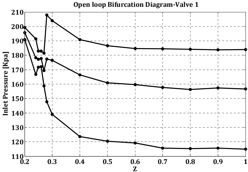
Figure 5.2: Open-loop bifurcation diagram from the slow choke valve experiments. The bifurcation point occurs at valve opening of Z=0.26 . The top and bottom line illustrate the maximum and minimum values of oscillations for inlet pressure respectively at each operating point. The middle line shows the average values of pressure.
