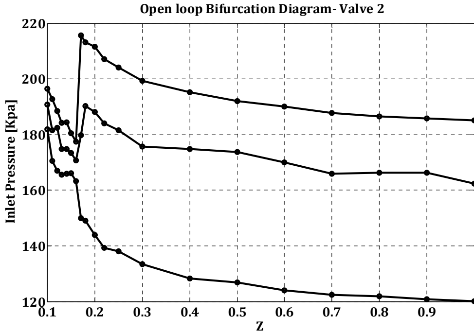
Figure 5.8: Open-loop bifurcation diagram from the fast choke valve experiments. The bifurcation point occurs at valve opening of Z=0.16 . The top and bottom line illustrate the maximum and minimum values of inlet pressure respectively at each operating point. The middle line shows the average values of pressure.
