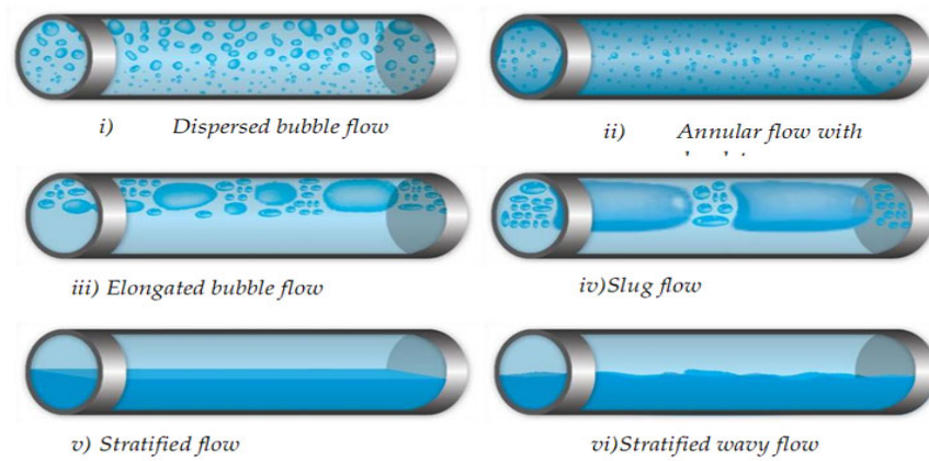
Figure 2.1: Gas-liquid flow regimes in horizontal pipes.
