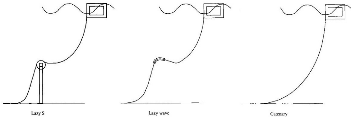
Figure 2.5: Common riser configurations applied in the oil and gas industry(Bai 2001)
