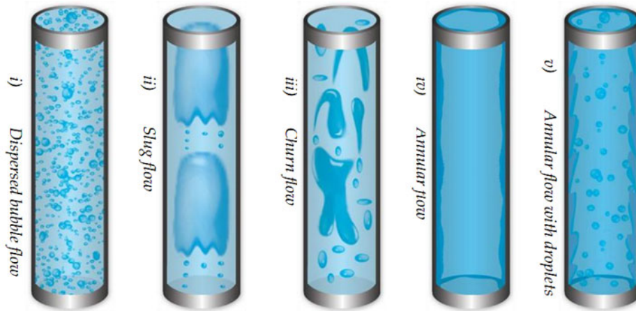
Figure 2.2: Gas-liquid flow regimes in vertical pipes. Slug flow is the point of interest in the thesis.
