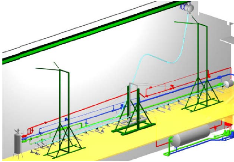
Figure 3.2: Multiphase Test Rig Layout, NTNU (Lilleby 2003)
