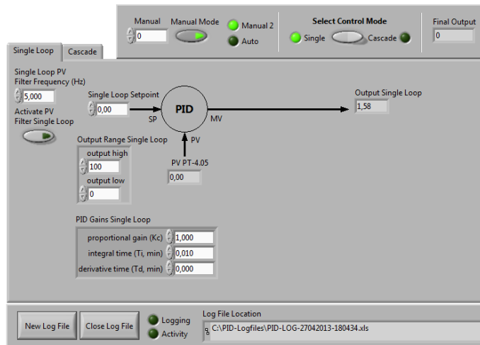
Figure 3.16: Implemented control modes in LabVIEW
