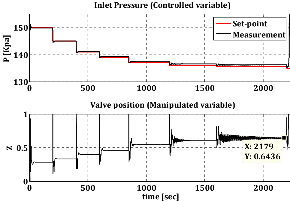
Figure 5.21: Simulation result of control by P-Only controller for K_c = 0.5 with OLGA. This has been the best result from trial and error due to the lowest achievable set-point or in other words the highest level of valve opening.
