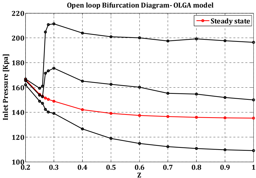
Figure 5.20: Open-loop bifurcation diagram from OLGA simulations. The bifurcation point occurs at valve opening of Z=0.26 . The top and bottom line illustrate the maximum and minimum values of oscillations for inlet pressure respectively at each operating point. The mid-black line is the shows the average values of pressure.
