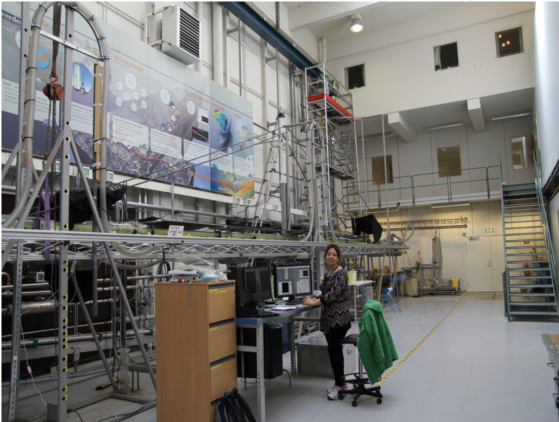
Figure 3.1: Medium scale experimental setup of multiphase flow laboratory located at department of Energy and Process Engineering of NTNU
