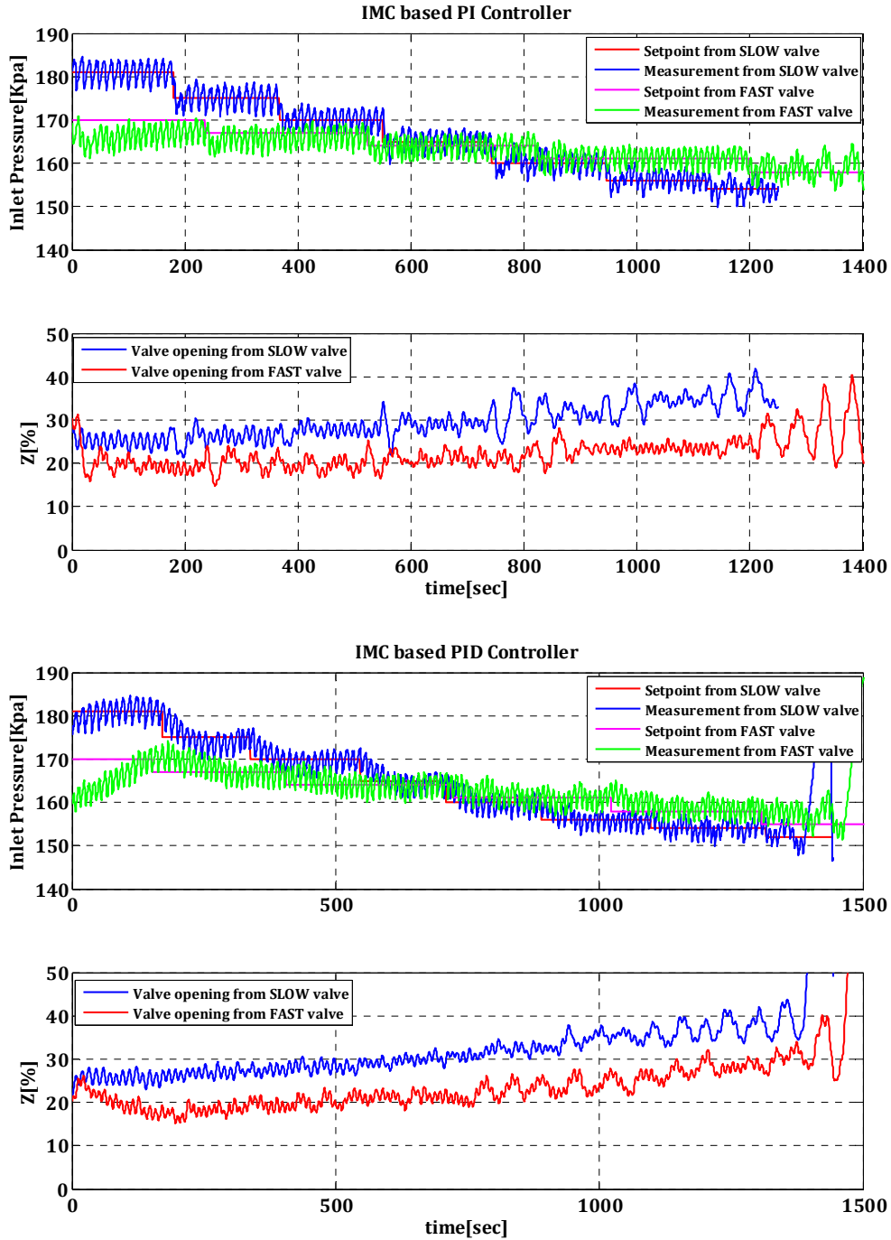
Figure 5.19: Comparison of IMC-based control results from slow valve with those of fast valve. With the slow valve it has been able to decrease set-point in a wider range to a lower level. With the fast valve, the open-loop system switched to slugging at P = 170 kpa while with the slow valve the instability started at P=180 kpa in the open-loop system. These are the initial points, respectively, to start control. The minimum achievable set-point has been P=154 kpa for the slow valve and P=158 kpa for the fast valve. This means that the slow valve has shown a better performance for the slugging system and has been already fast enough as well.
