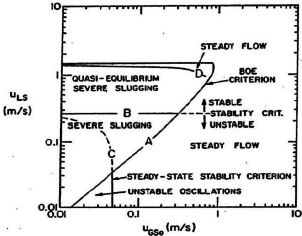
Figure 2.3: Stability map for multiphase flow (Taitel 1986). Stability boundaries are clearly shown in the map.
