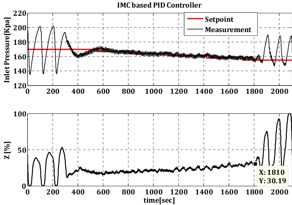
Figure 5.11: Result of control using the IMC-based PID controller. The controller has been able to move the bifurcation point from Z=16\% up to Z=30.19\% (about the double value).
