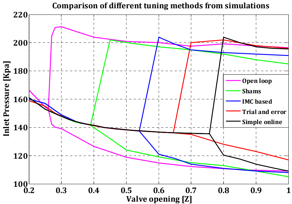
Figure 5.38: Comparison of stabilizing control results from different tuning methods applied in the simulations. It can be said that simple online method with gain scheduling is the most stabilizing and the IMC-based designed method is the second best as systematic manners to tune the controllers.
