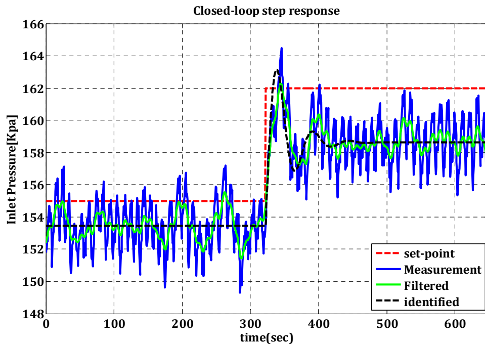
Figure 5.10: Presentation of identified closed-loop step response. The dashed black line shows the identified closed-loop transfer function obtained from IMC design.
