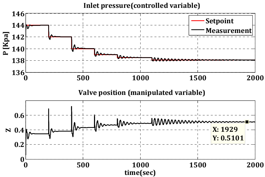
Figure 5.33: Simulation result of control using the IMC-based PI controller tuned at the initial choke valve position of Z=40\% .
