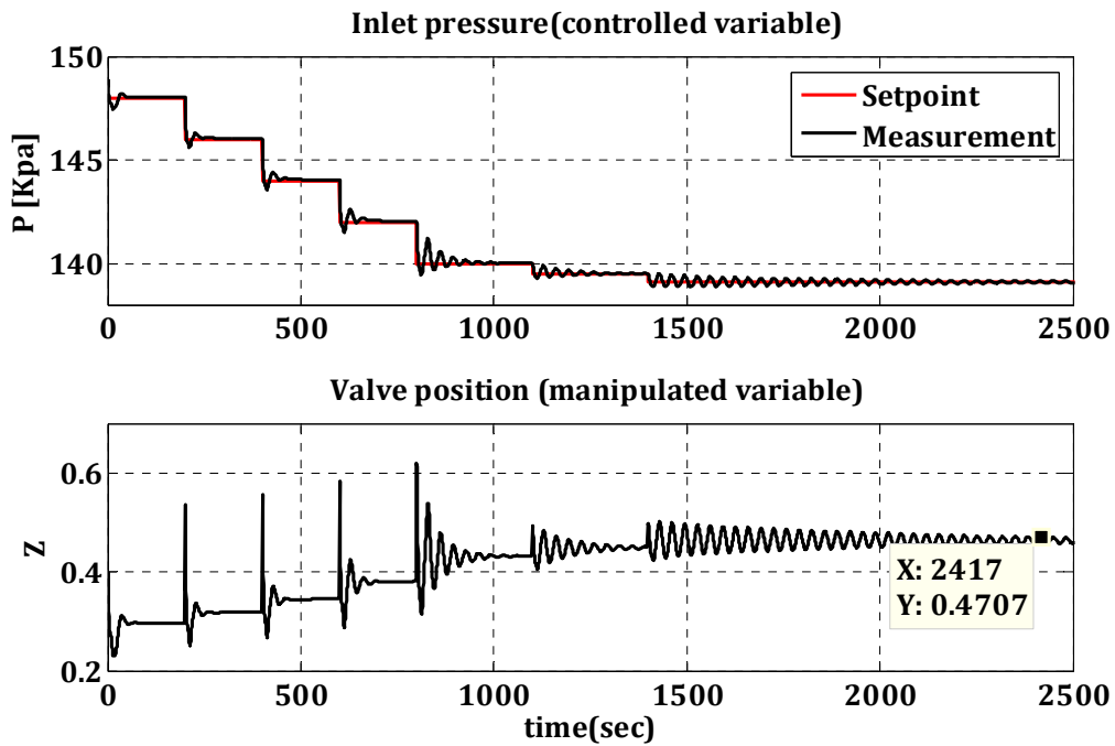
Figure 5.30: Simulation result of control using the IMC-based PI controller tuned at the initial choke valve position of 30%.
