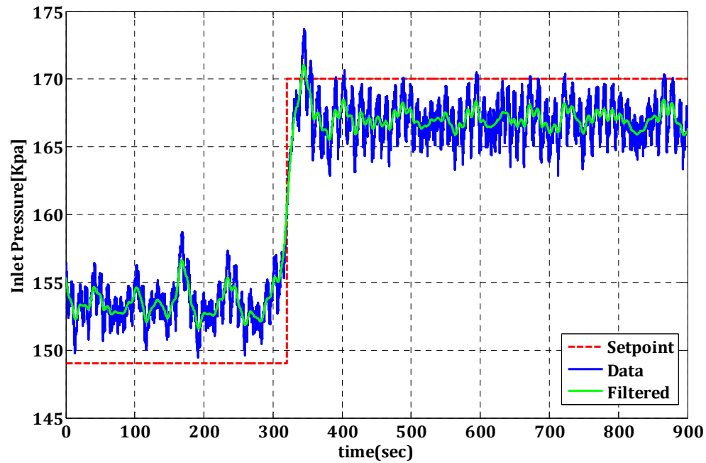
Figure 5.4: Set-point step change for a closed-loop feedback experiment with a P_only controller using inlet (buffer) pressure as control variable. A low pass filter with a smoothing factor of \alpha = 0.001 was used to remove the noise effect from the response.
