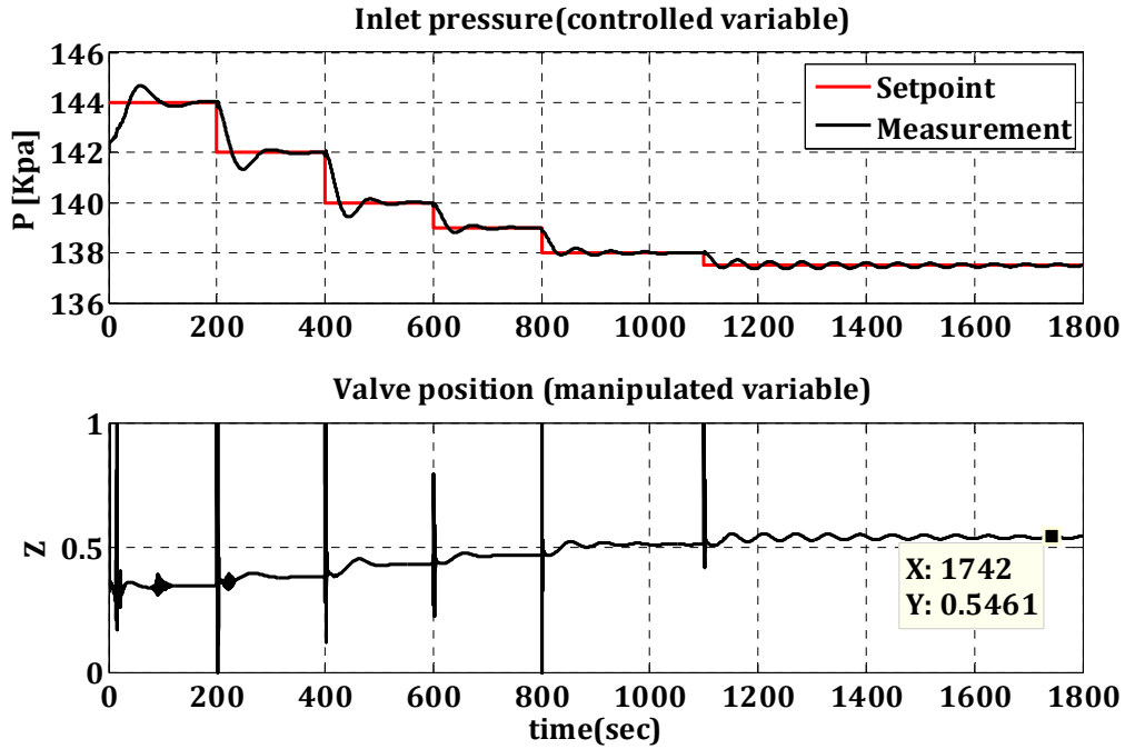
Figure 5.32: Simulation result of control using the IMC-based PID controller tuned at the initial choke valve position of Z=40\% .
