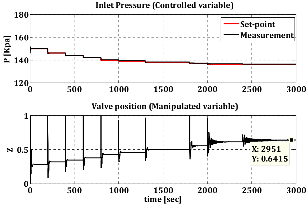
Figure 5.23: simulation results of control by PI controller for K_c = 0.5 and \tau_i = 800
