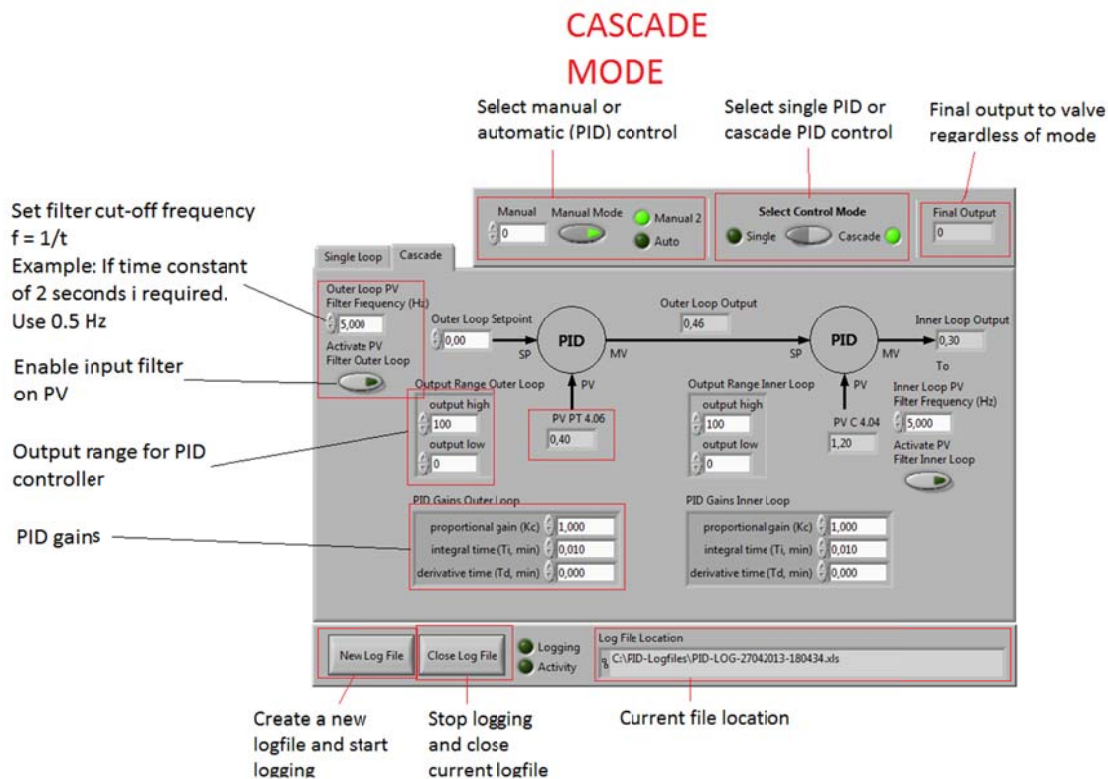
Figure 5.15: A schematic view of cascade control structure in LabVIEW. The outer loop receives signal from top pressure sensor as the measurement and produces the setpoint signal for the inner loop. The inner loop uses the density signal from the conductance probe installed in the outlet of the riser.
