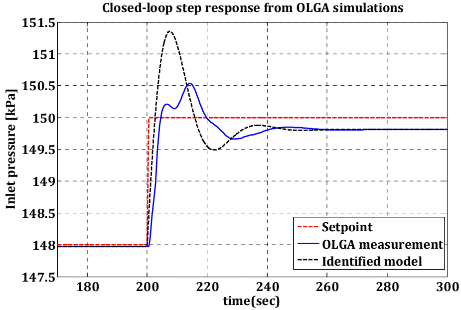
Figure 5.28: Closed-loop response of step change at initial valve opening Z=0.3 . The dashed black line shows the transfer function of the IMC-based identified model.
