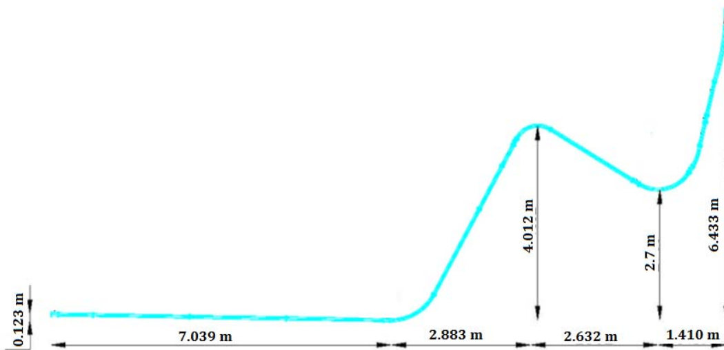
Figure 3.4: Configuration of the S-shaped riser test section (Lilleby 2003)
